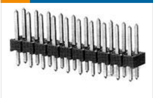
TE Part #3-826632-6 36P AMPMODU II STIFT LEI
