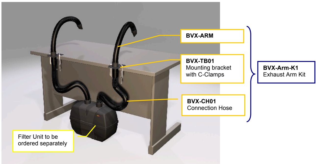
Fume Extraction Station using two BVX-ARM-K1 Kits
