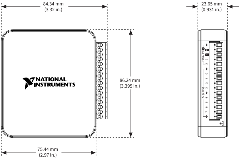
Figure 1. USB-6000 Dimensions
