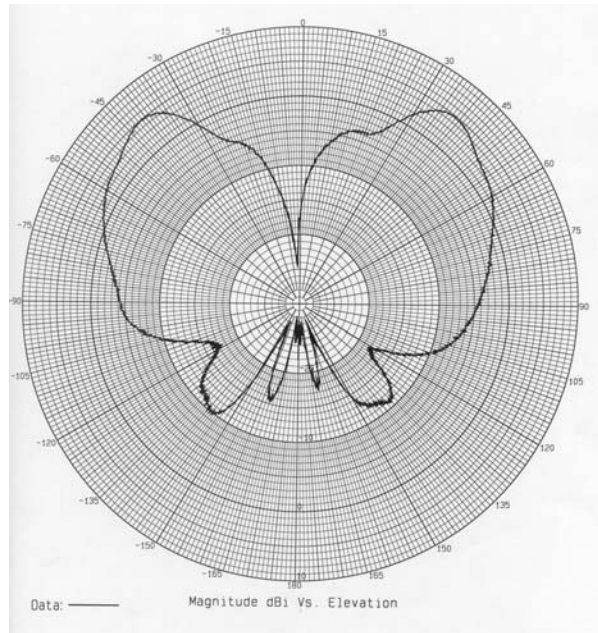
MGRM-WHF-XX at 5800 MHz – Elevation
