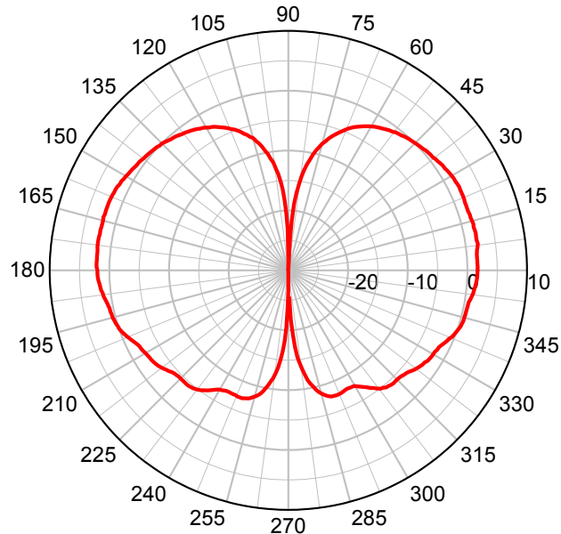
PSKN3-2400 Series – Elevation Plot
