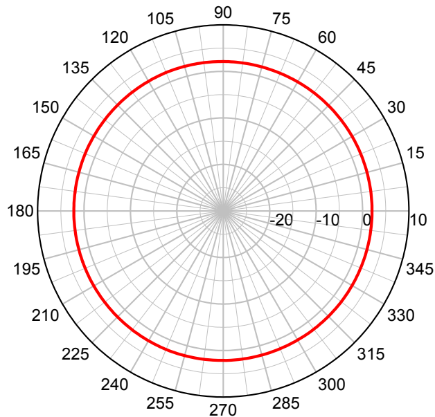
PSKN3-2400 Series – Azimuth Plot
