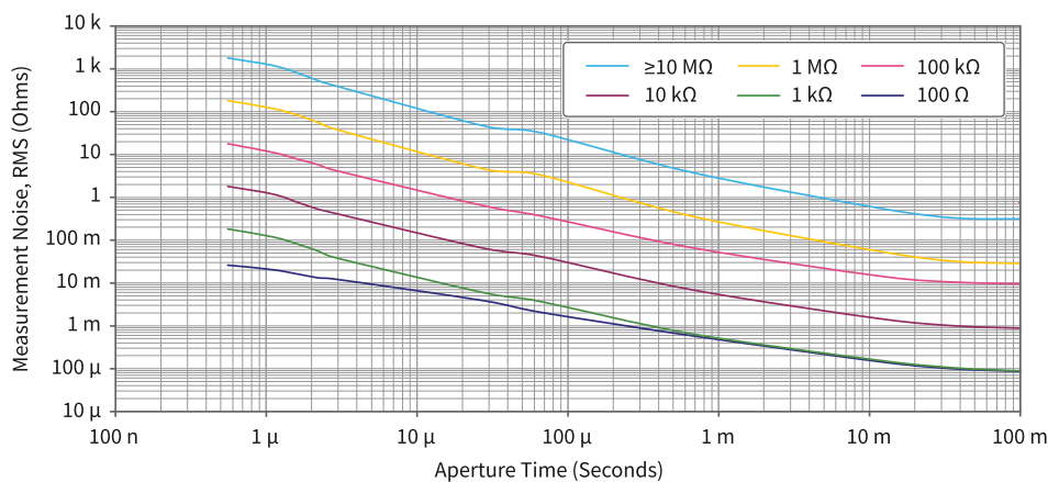
Figure 2. PXIe-4081 Resistance Noise, Typical
