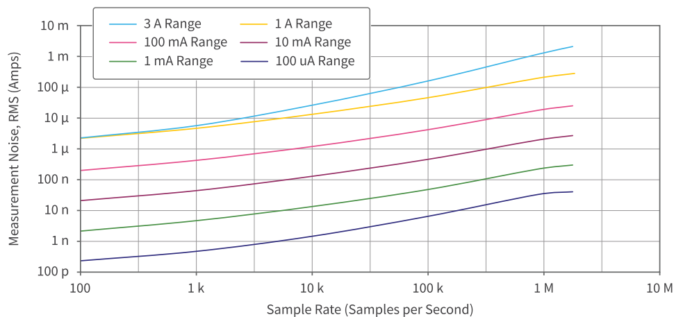
Figure 5. PXIe-4081 Current Waveform Noise with Input Open, Typical
