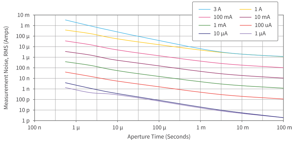
Figure 3. PXIe-4081 DC Current Noise, Typical
