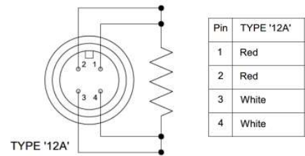
4 pin Wiring Diagram.
