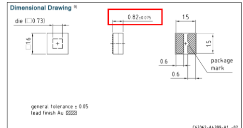
Device height: 0.82 \pm 0.075 mm
