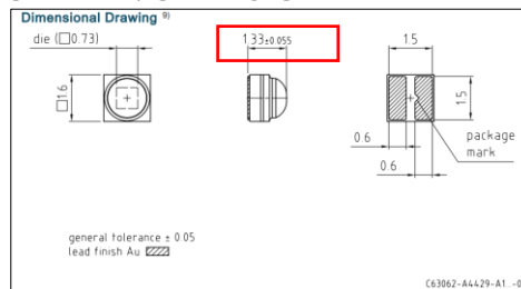
Device height: 1.33 \pm 0.055 mm
