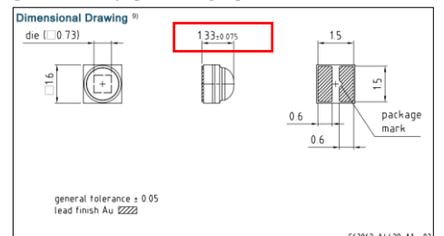
Device height: 1.33 \pm 0.075 mm
