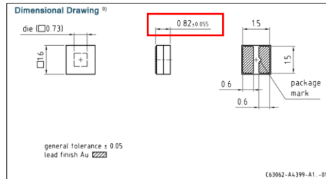
Device height: 0.82 \pm 0.055 mm
