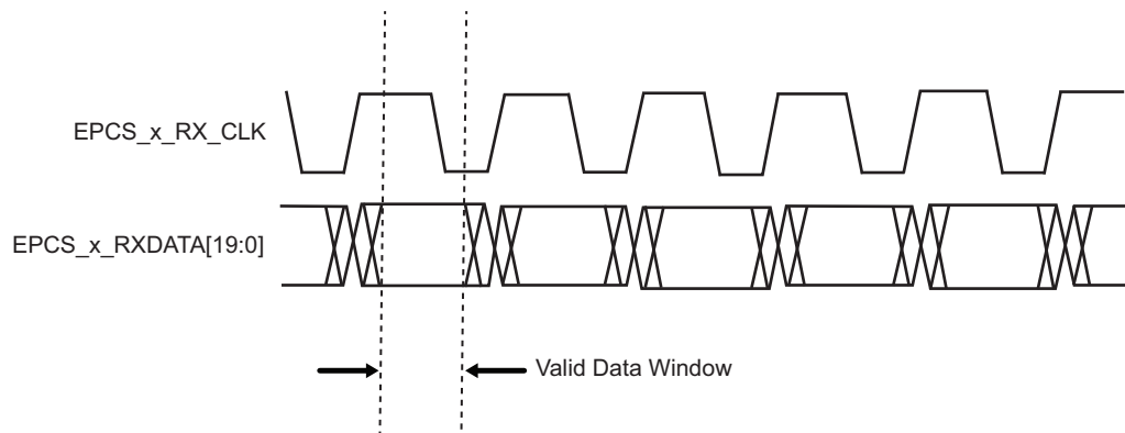
Figure 6-12. EPCS Receive Interface Timing Diagram
