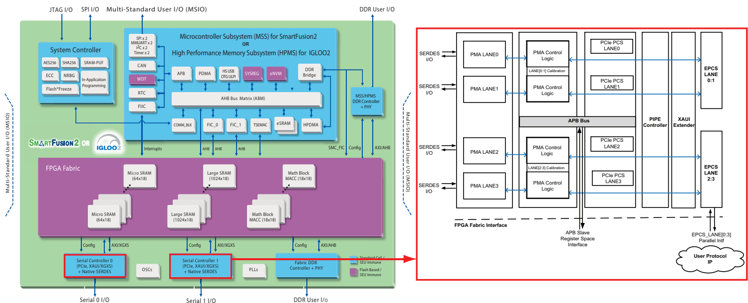
Figure 6-1. SmartFusion 2 and IGLOO 2 SERDESIF Block Diagram
