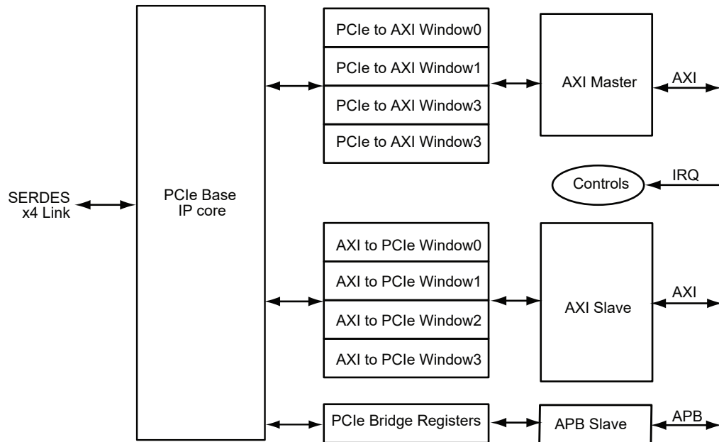
Figure 4-11. PCIe Hard Block Diagram
