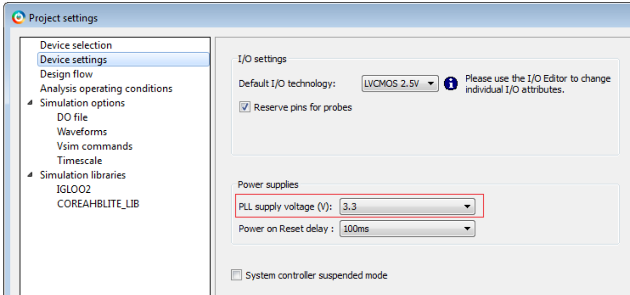
Figure 3-4. SPL Power Supply Selection in the Libero® SoC New Project Wizard
