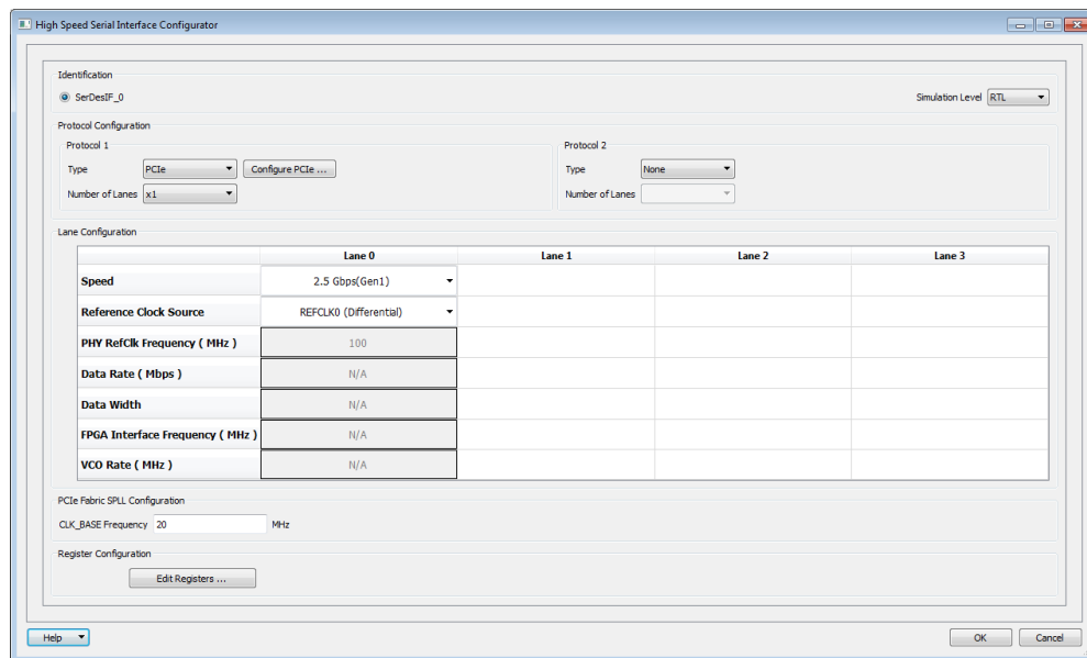
Figure 3-2. Libero® SoC SERDESIF GUI
