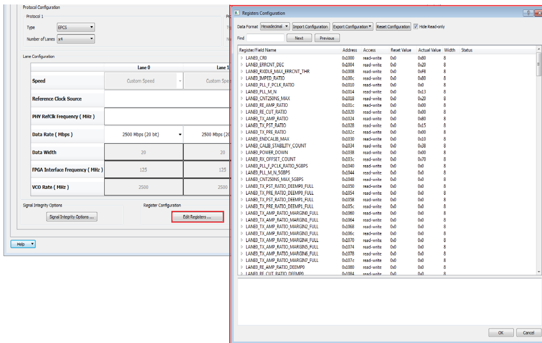
Figure 6-14. SERDESIF Configurator Window
