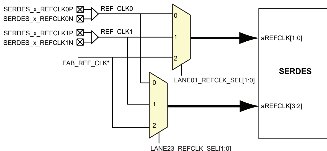
Figure 4-14. SerDes Reference Clock for PCIe Mode
