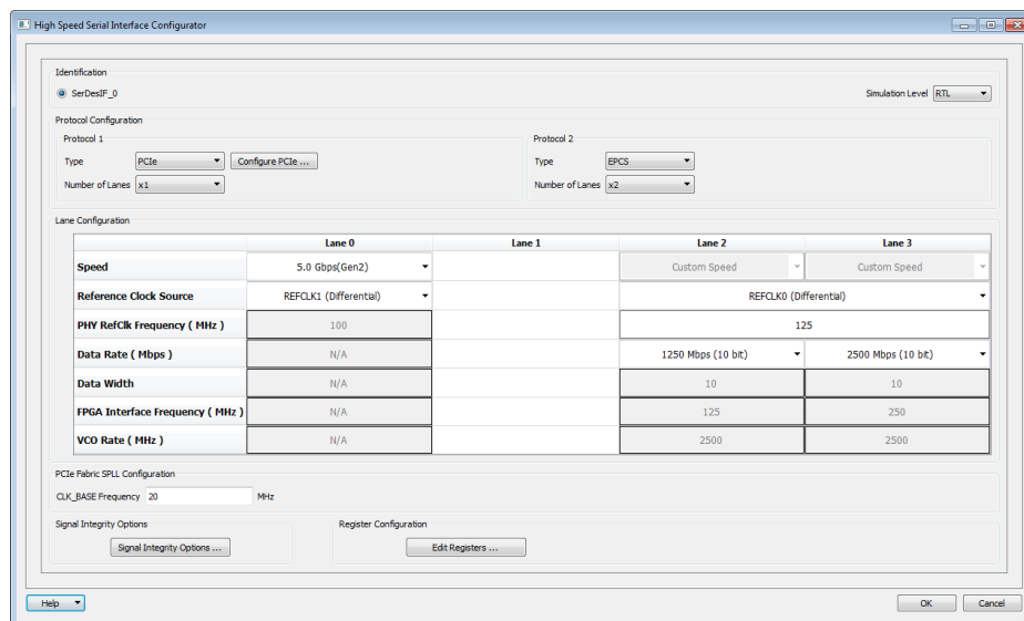
Figure 6-5. EPCS Custom Speed Mode in SERDESIF Configurator
