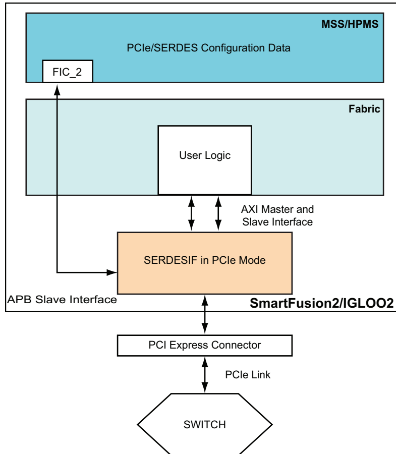
Figure 4-3. SmartFusion® 2 and IGLOO® 2 PCIe EP Implementation
