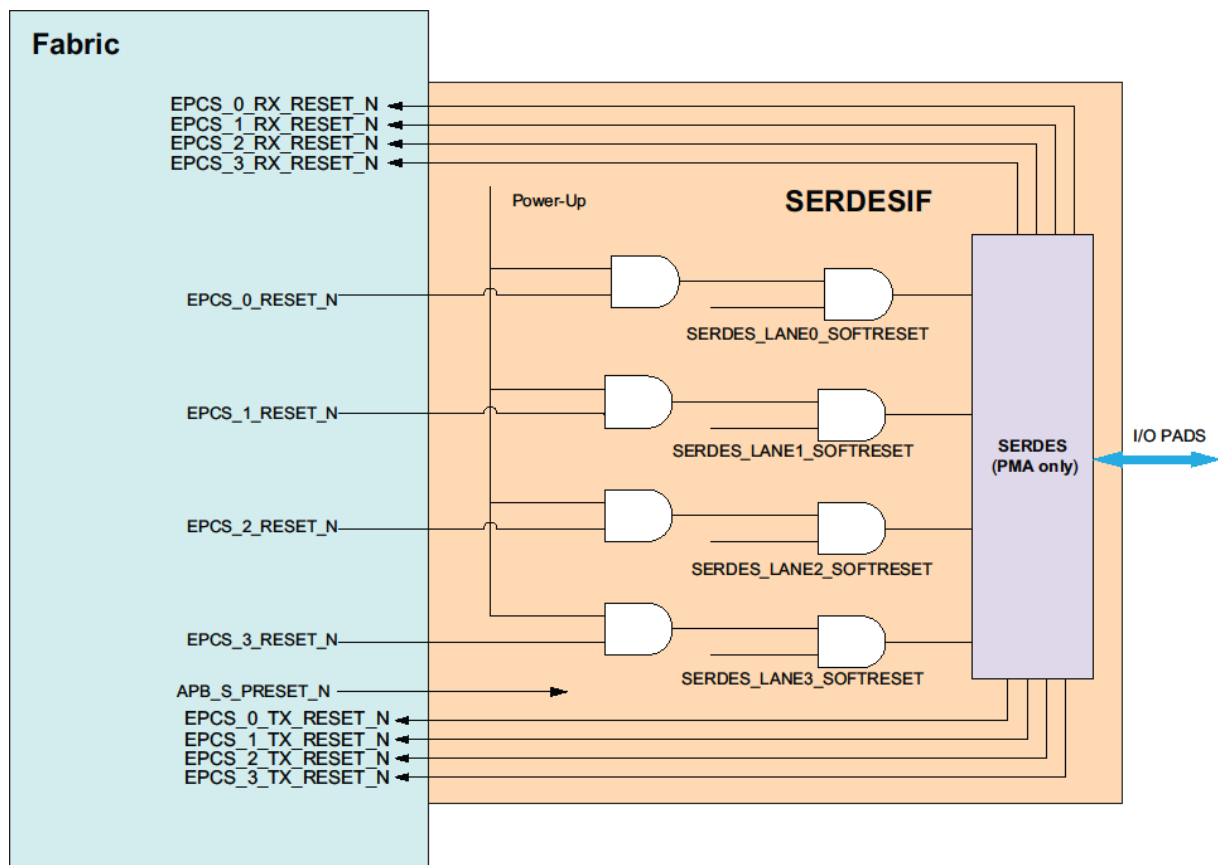
Figure 6-10. SERDESIF Reset Signals in EPCS Mode
