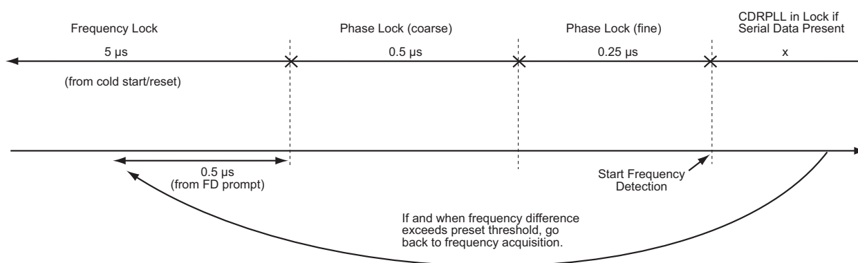
Figure 7-18. CDR Bit Locking
