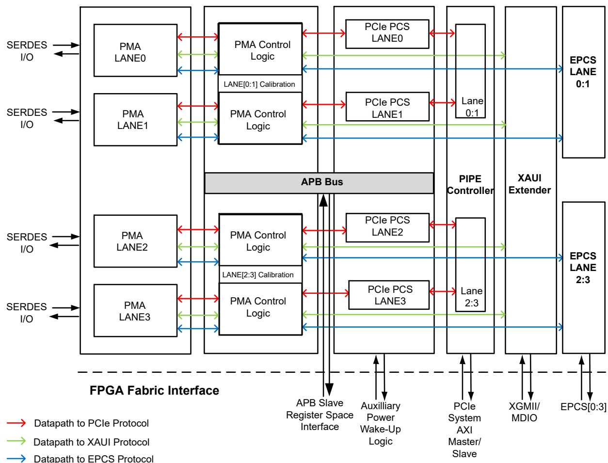
Figure 1. SmartFusion® 2 and IGLOO® 2 SERDESIF Block Diagram
