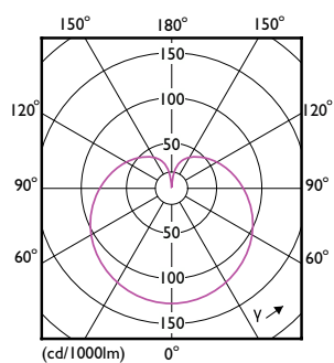
Light Distribution Diagram - CorePro LEDbulb ND 5-40W A60 B22 930
