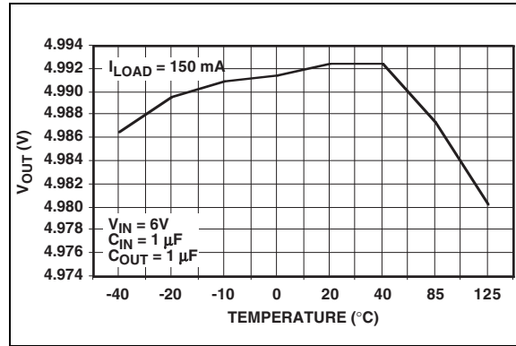
FIGURE 2-14: Output Voltage vs. Temperature ( V_{OUT} = 5 \text{ V} ).
