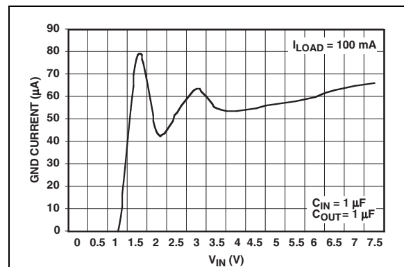
FIGURE 2-6: Ground Current vs. V_{IN} ( V_{OUT} = 3.3\text{V} ).
