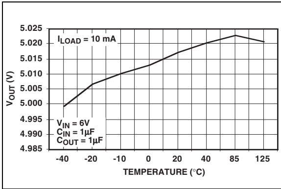
FIGURE 2-12: Output Voltage vs. Temperature ( V_{OUT} = 5 \text{ V} ).
