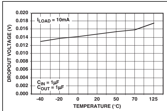
FIGURE 2-1: Dropout Voltage vs. Temperature ( V_{OUT} = 3.3\text{V} ).
