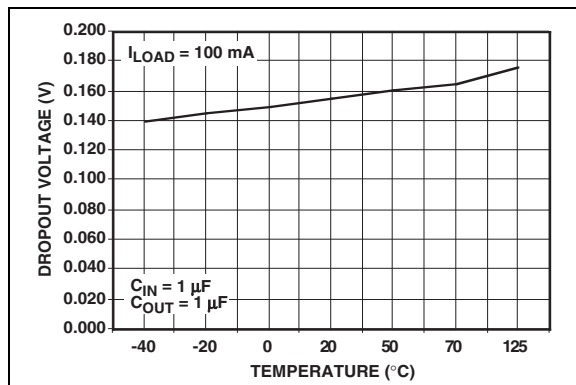
FIGURE 2-2: Dropout Voltage vs. Temperature ( V_{OUT} = 3.3\text{V} ).
