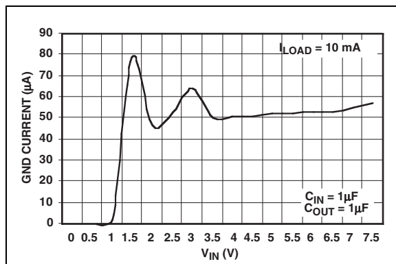
FIGURE 2-3: Ground Current vs. V_{IN} ( V_{OUT} = 3.3\text{V} ).
