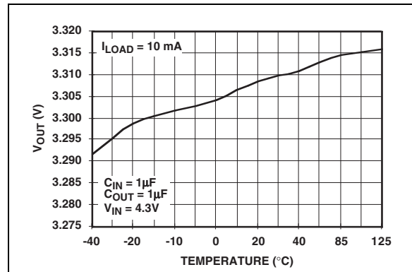
FIGURE 2-11: Output Voltage vs. Temperature ( V_{OUT} = 3.3V ).
