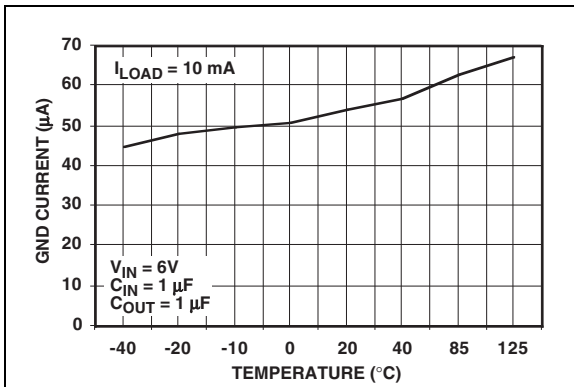
FIGURE 2-13: Temperature vs. Quiescent Current ( V_{OUT} = 5 \text{ V} ).
