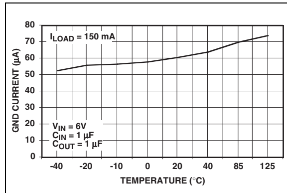
FIGURE 2-15: Temperature vs. Quiescent Current ( V_{OUT} = 5 \text{ V} ).
