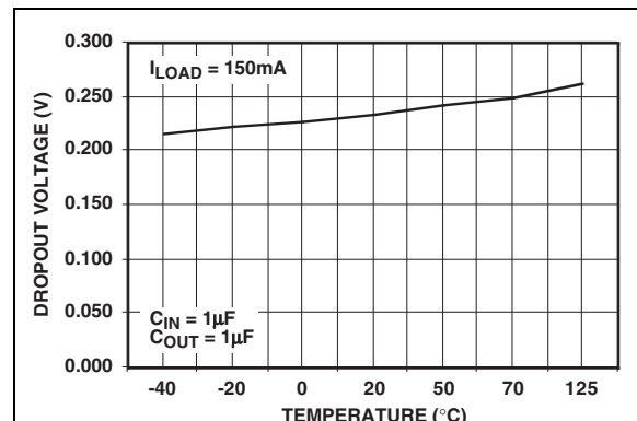
FIGURE 2-5: Dropout Voltage vs. Temperature ( V_{OUT} = 3.3\text{V} ).
