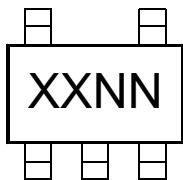
5-Lead SOT-23-5
