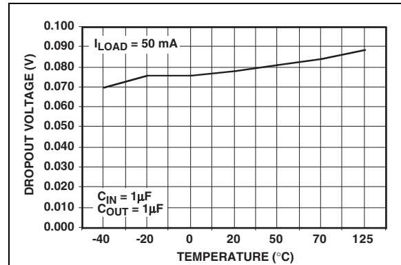
FIGURE 2-4: Dropout Voltage vs. Temperature ( V_{OUT} = 3.3\text{V} ).
