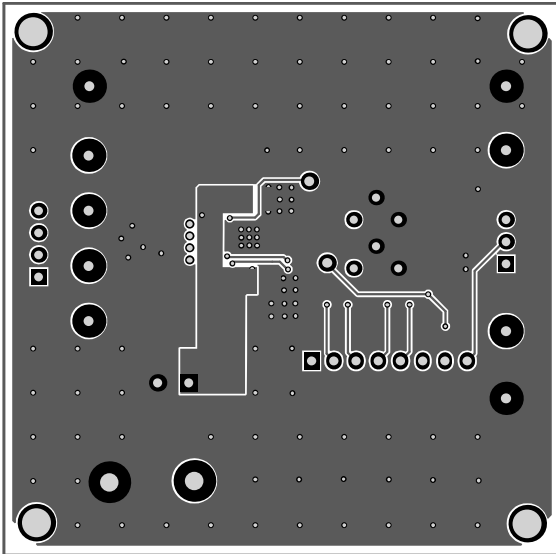
Figure 4: Bottom Layer
