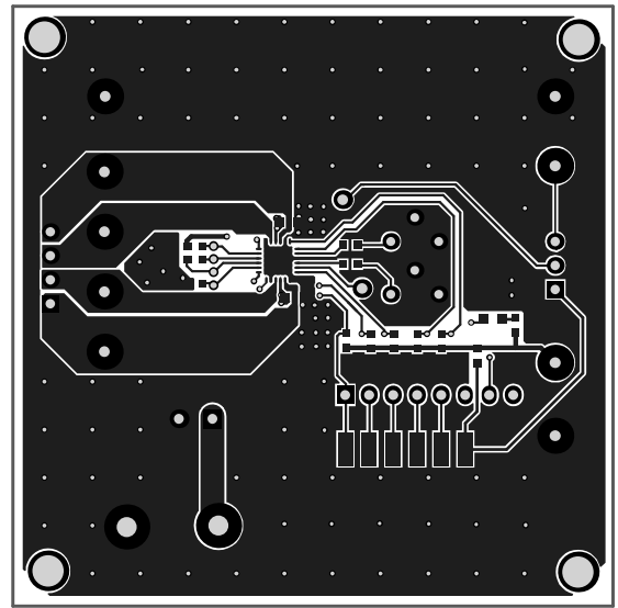
Figure 3: Top Layer
