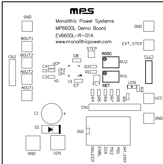
Figure 2: Top Silk
