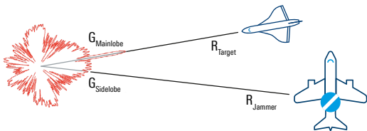
Fig. 20: Support jamming
