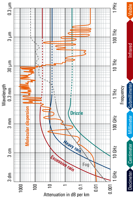
Fig. 10: Atmospheric and rain attenuation
