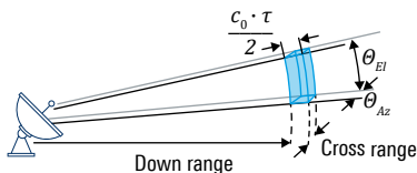
Fig. 34: Point-like targets
