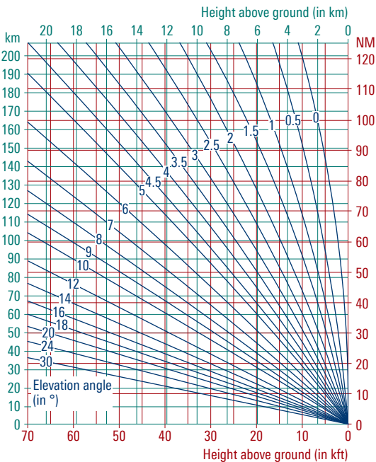
Fig. 32: Influence of refractions on range of radio horizon
