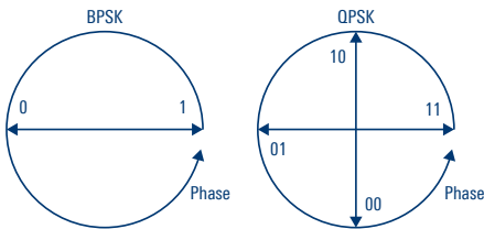
Fig. 24: BPSK and QPSK
