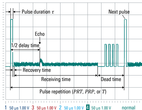
Fig. 21: Pulse repetition time
