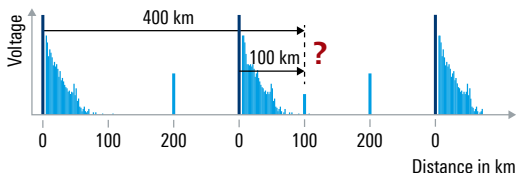
Fig. 22: Radar unambiguous range
