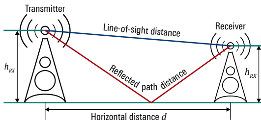
Fig. 12: LOS and reflected path distances
