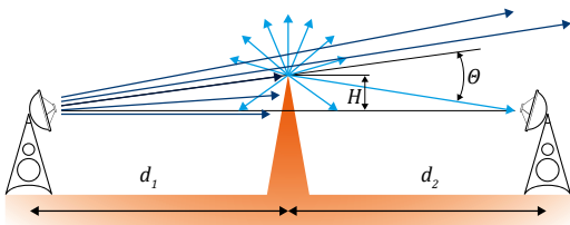
Fig. 13: Knife edge diffraction
