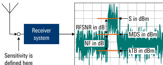
Fig. 15: Definition of receiver sensitivity
