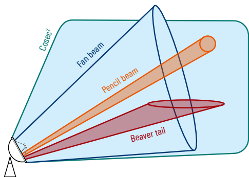
Fig. 14: Radar antenna patterns at a glance
