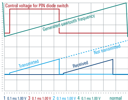
Fig. 28: FMiCW radar
