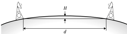
Fig. 9: Relation of earth bulge and link distance
