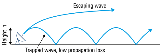
Fig. 33: Ducting
