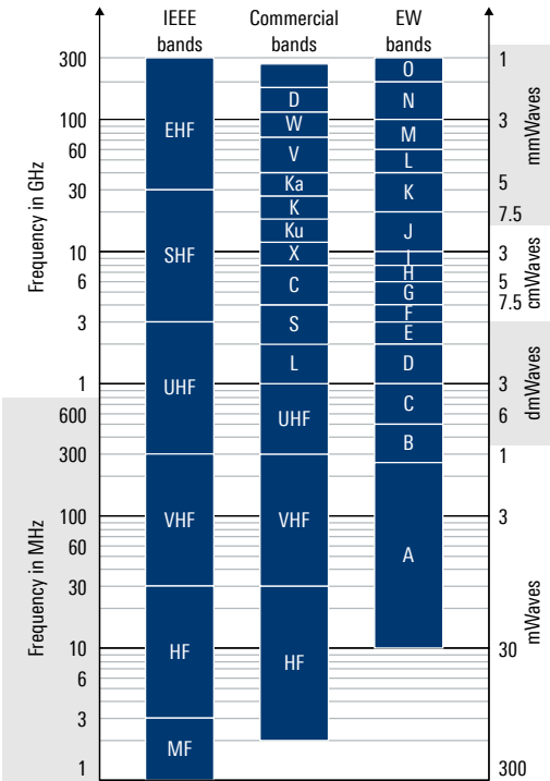
Fig. 1: Frequency bands from 1 MHz to 300 GHz
