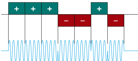
Fig. 25: Bi-phase PMOP Barker code
