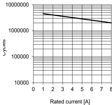
Characteristically electrical endurance acc. IEC60947-5-1 DC-1 Ue=24VDC
