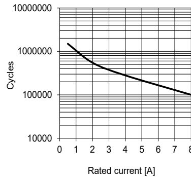
Characteristically electrical endurance acc. IEC60947-5-1 AC-1 Ue=250VAC 85°C
