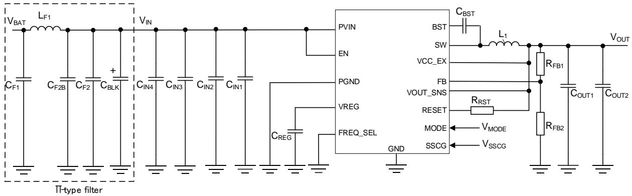
Figure 66. Reference Circuit 3
