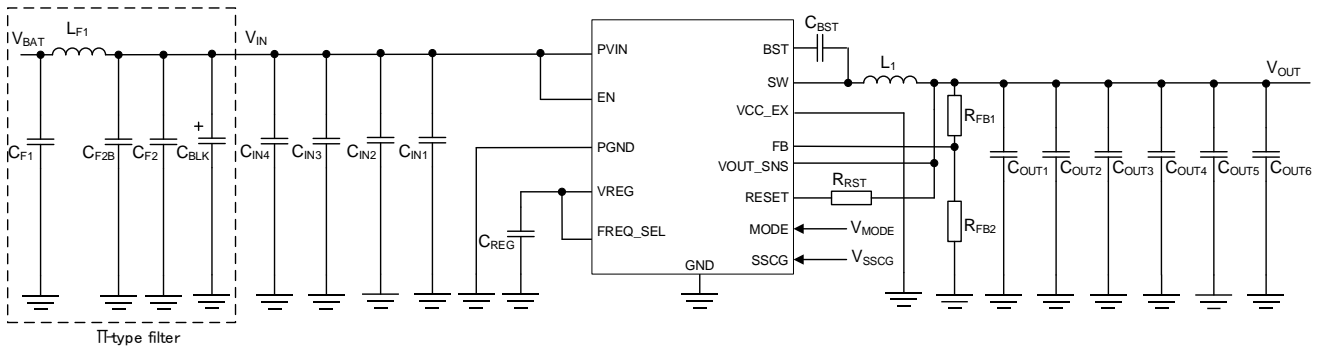
Figure 53. Reference Circuit 2
