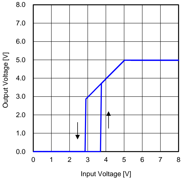
Figure 75. Output Voltage vs Input Voltage 1 (R LOAD = 166 Ω)
