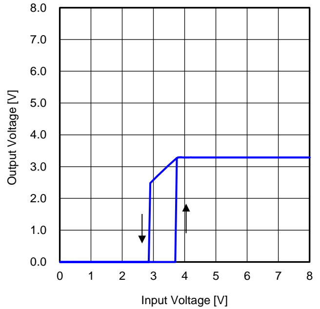
Figure 50. Output Voltage vs Input Voltage 2 ( R_{LOAD} = 0.55 \Omega )
