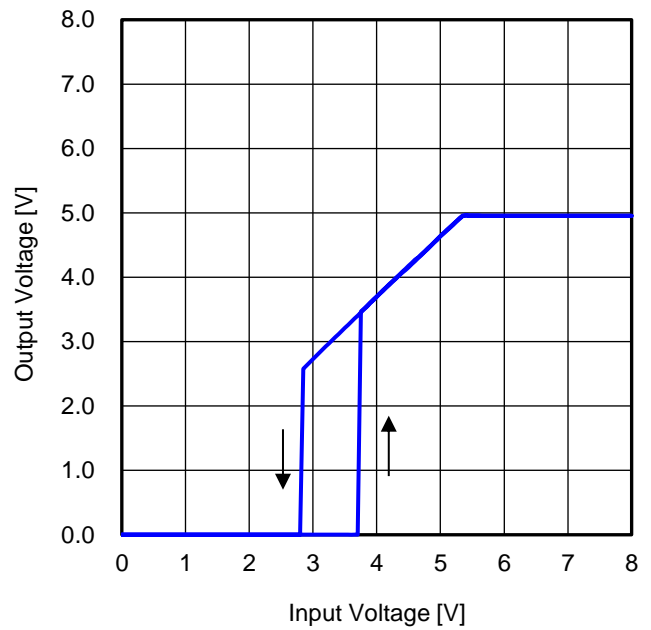
Figure 76. Output Voltage vs Input Voltage 2 (R LOAD = 0.83 Ω)
