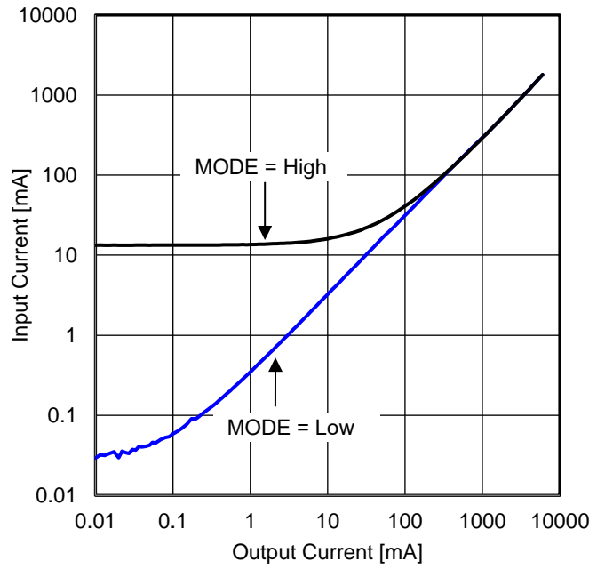
Figure 55. Input Current vs Output Current (VIN = 12 V)
