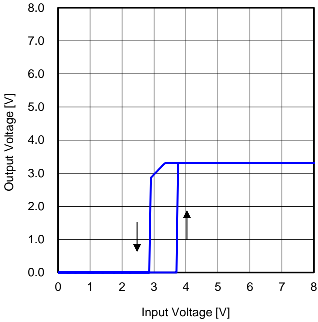
Figure 49. Output Voltage vs Input Voltage 1 ( R_{LOAD} = 110 \Omega )
