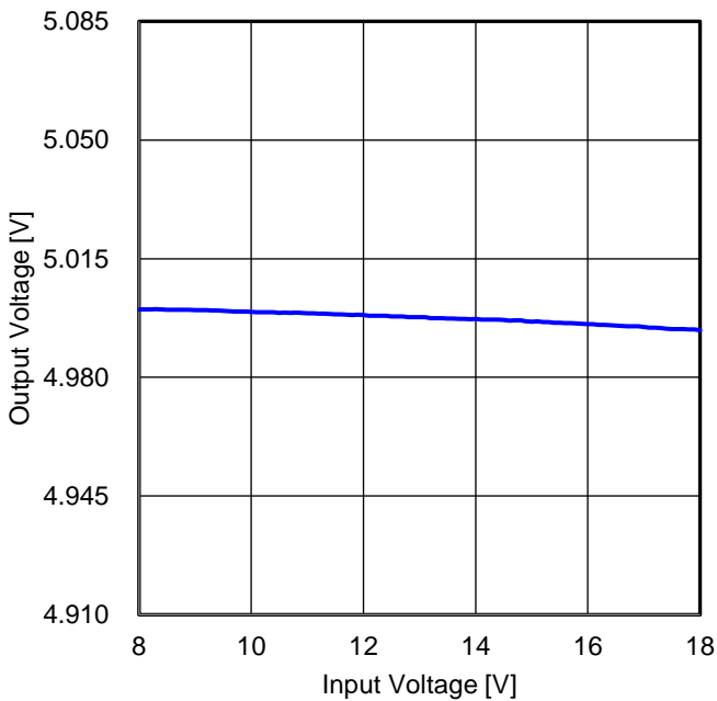
Figure 77. Line Regulation (I OUT = 3 A)
