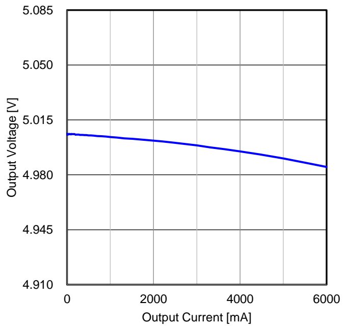
Figure 78. Load Regulation (V IN = 12 V)
