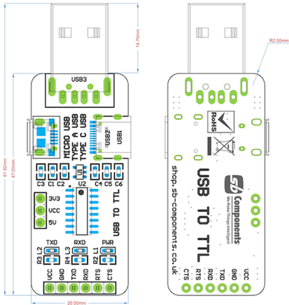
CH340 Front and Back Images
