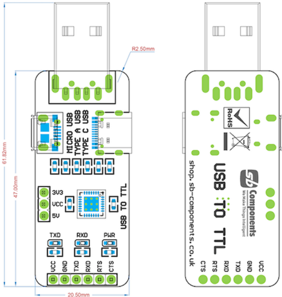
CP2102 Front and Back Images
