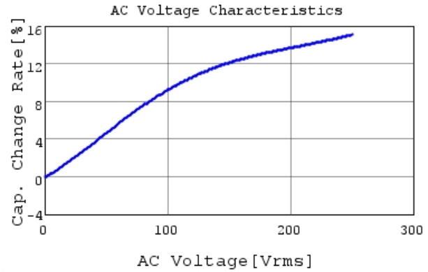
DE2B3SA101KN2AT01F C-AC Voltage capchange, I
