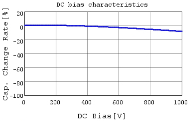
DE2B3SA101KN2AT01F C-DC bias capchange, 20.0
