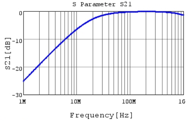
DE2B3SA101KN2AT01F S21 DCOV, 20degC
