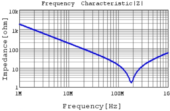
DE2B3SA101KN2AT01F |Z| DCOV, 20degC
