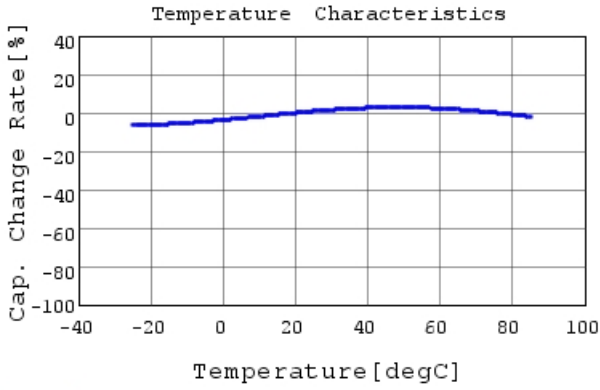
DE2B3SA101KN2AT01F C-Temp. capchange, DCOV,
