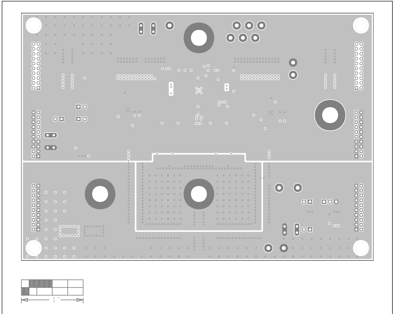
EV Kit PCB Layout—Internal Layer 2
