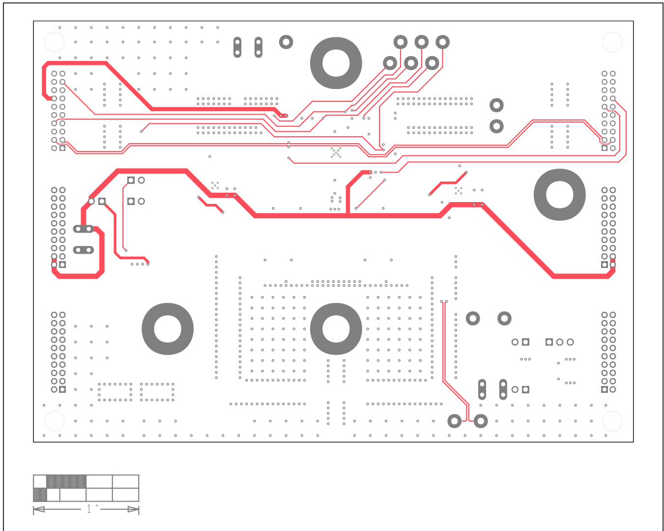
EV Kit PCB Layout—Internal Layer 4
