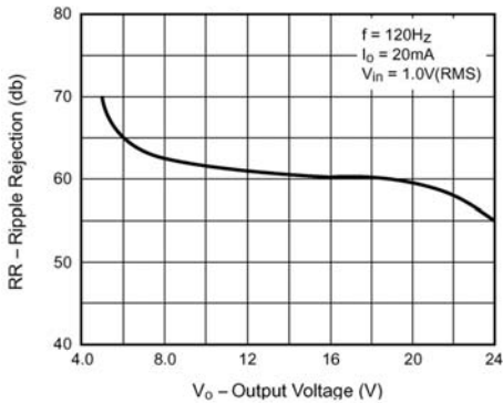
FIG. 5 - Ripple Rejection vs. Output Voltage
