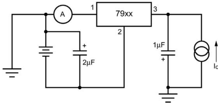
Test Circuit 2
