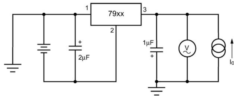
Test Circuit 3
