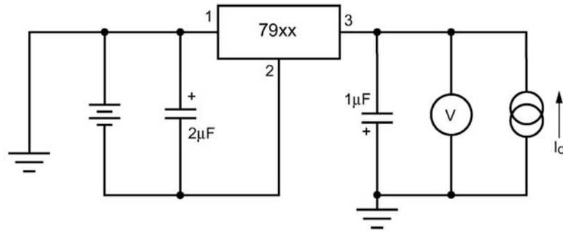
Test Circuit 1
