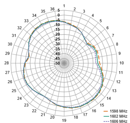
XY-Plane Gain
