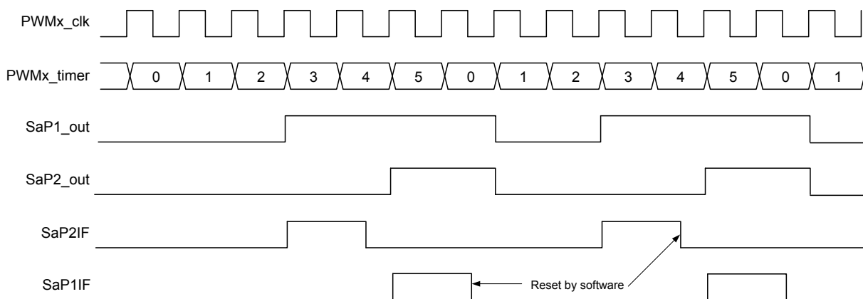
Figure 31-4. Right-Aligned Timing Diagram
