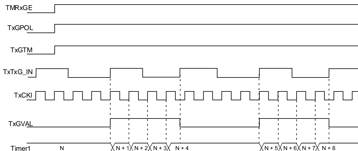
Figure 25-5. Timer1 Gate Toggle Mode
