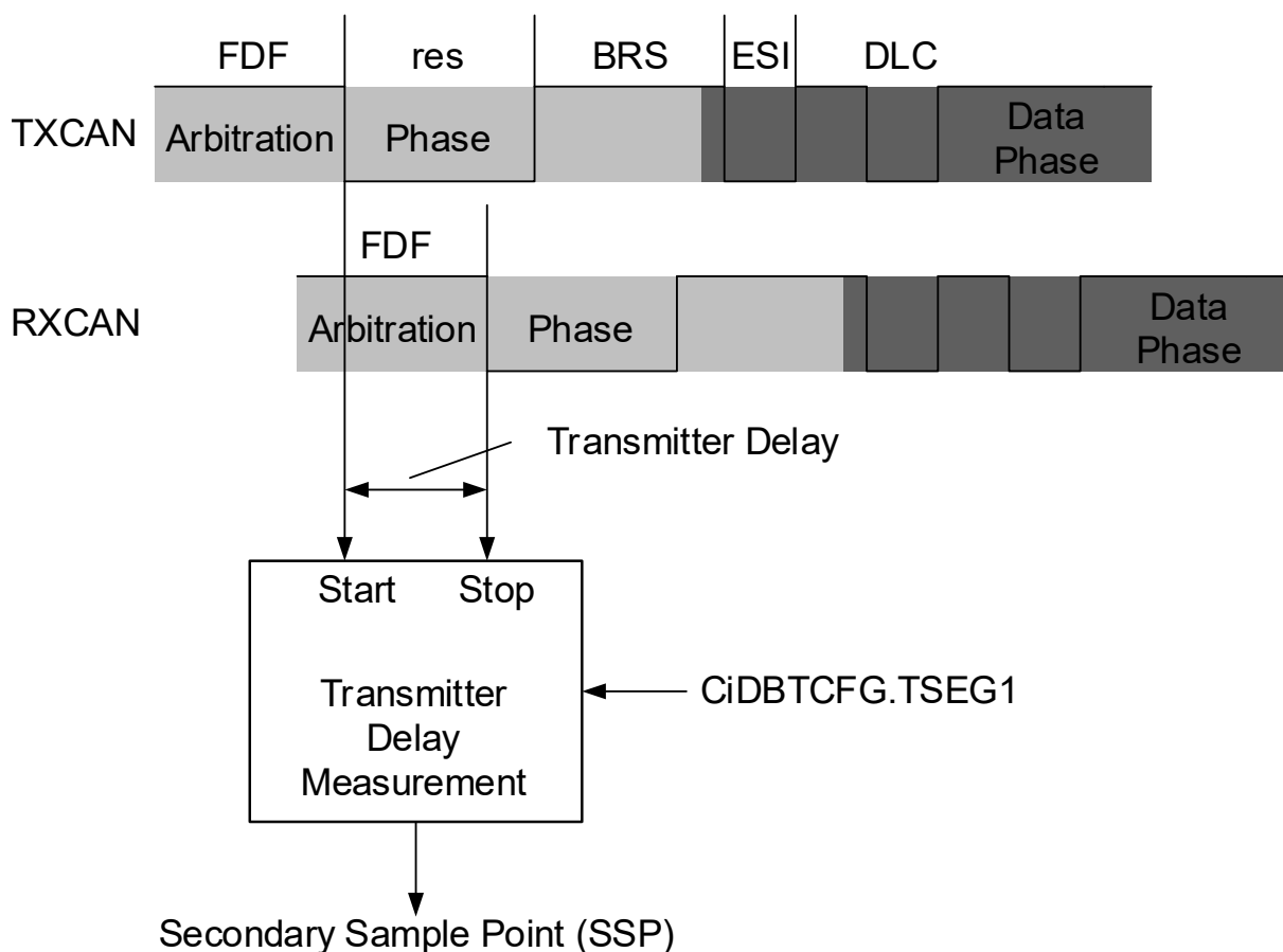
Figure 38-5. Measurement of Transceiver Delay (TDCV)
