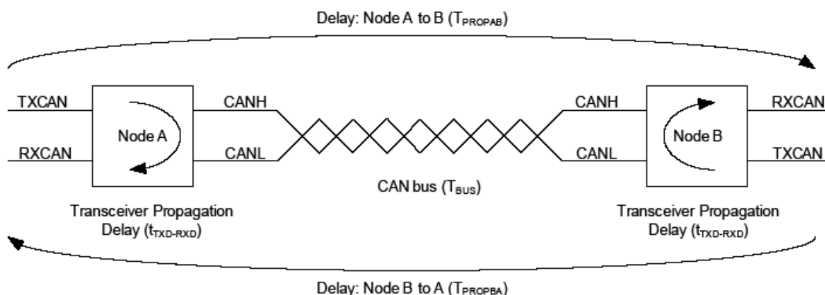
Figure 38-4. Propagation Delay
