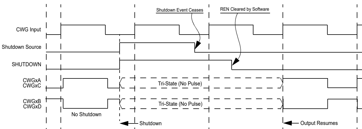
Figure 32-15. Shutdown Functionality, Auto-Restart Disabled (REN = 0, LSAC = 'b01, LSB0 = 'b01)
