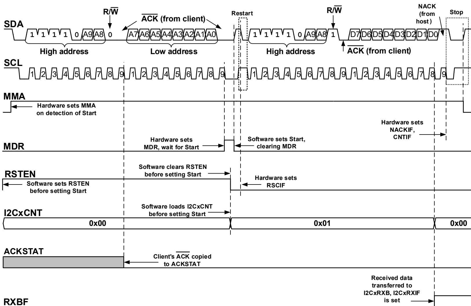
Figure 37-40. 10-Bit Host Mode Reception
