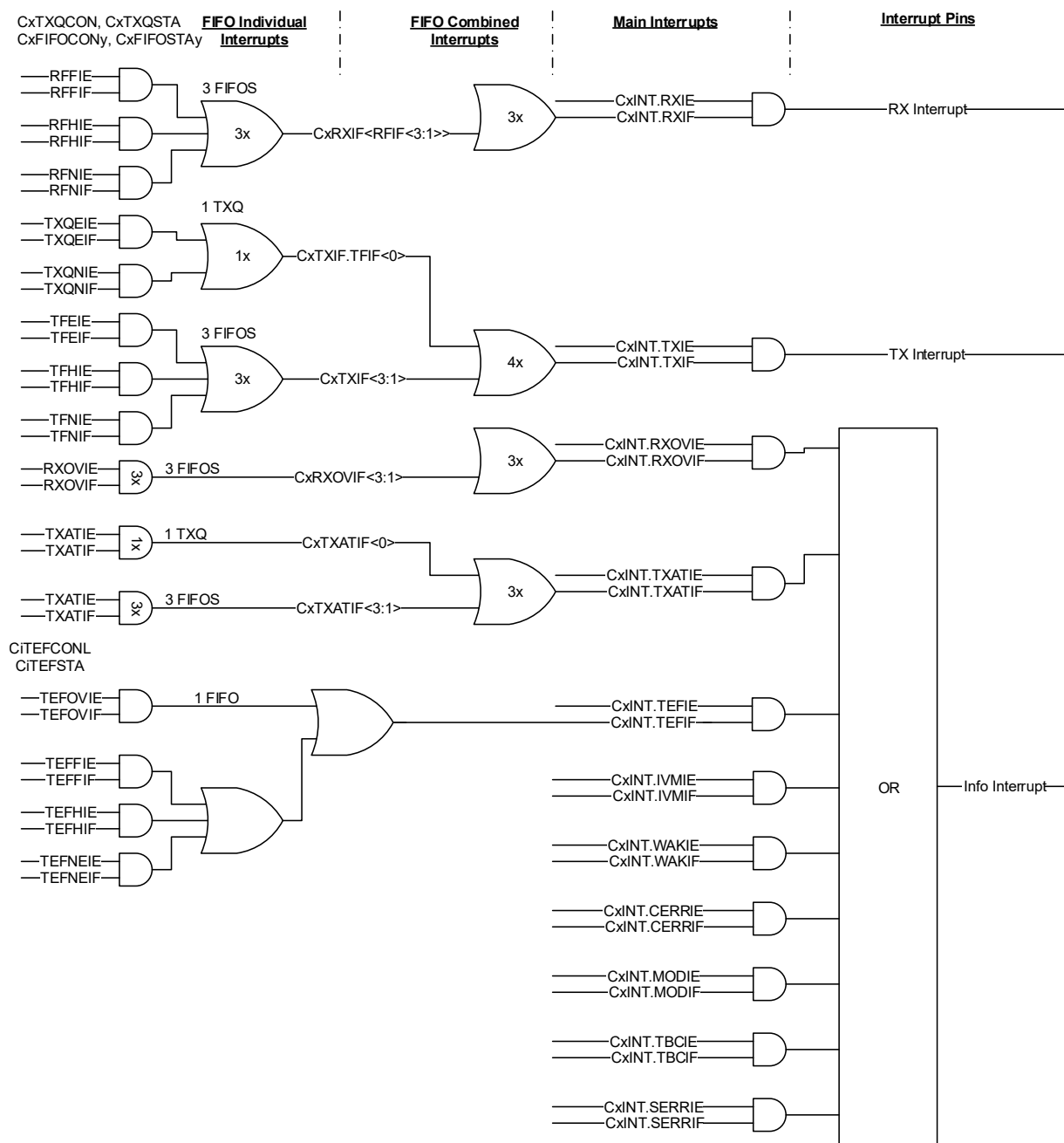
Figure 38-46. Interrupt Multiplexing
