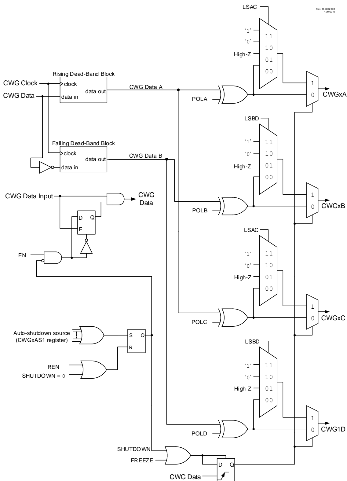
Figure 32-2. Simplified CWG Block Diagram (Half Bridge Mode, MODE = 'b100)
