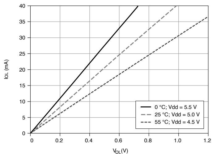
Figure 4. P0.<0..7>: I_{OL} versus V_{OL}
