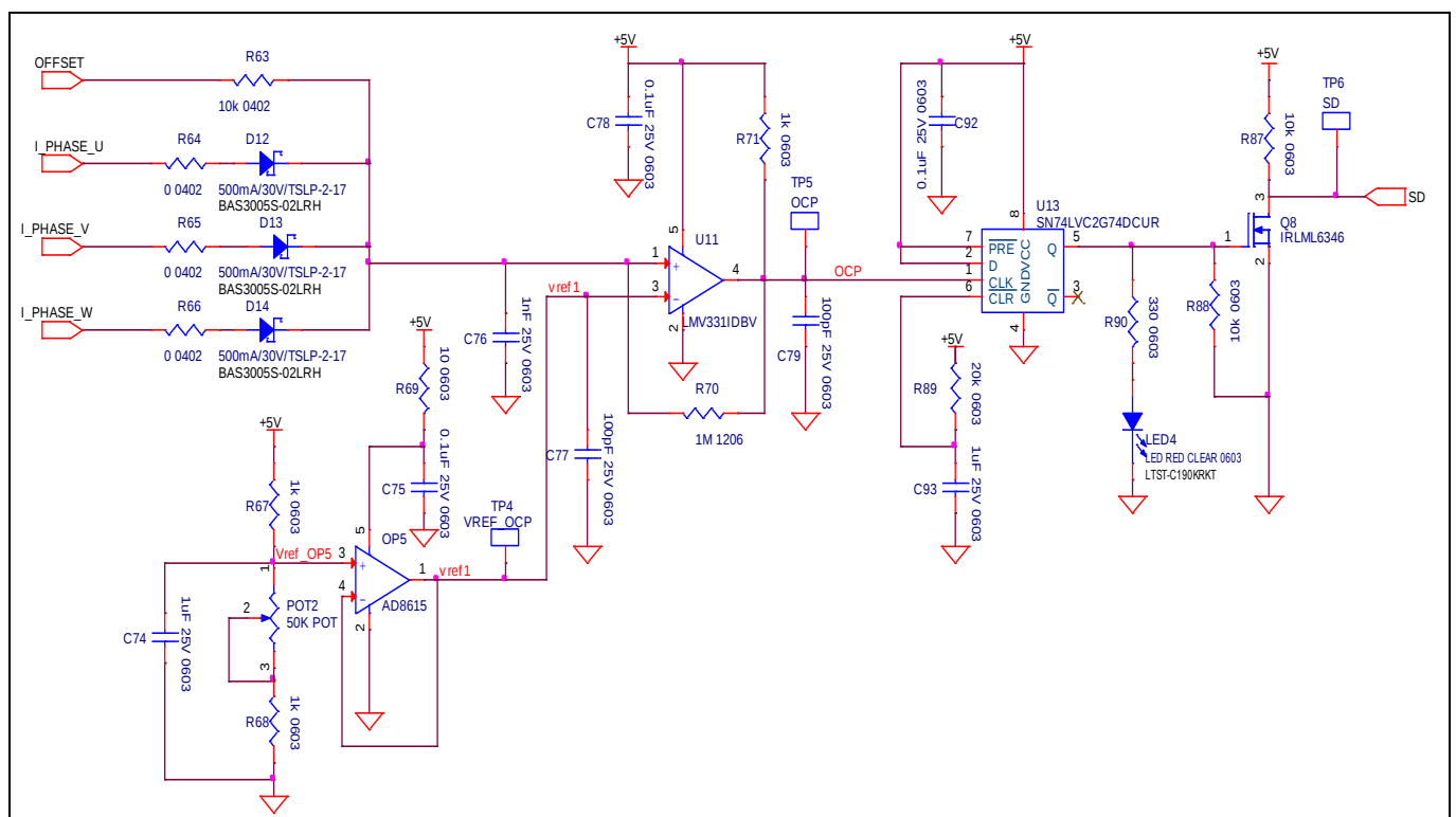
Figure 17 OCP circuitry
