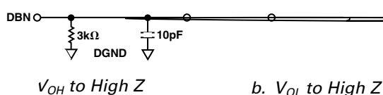
Figure 2. Load Circuits for Bus Relinquish Time ( t_7 )
