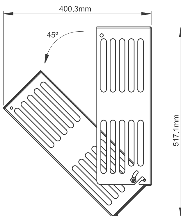
OPEN SIDE VIEW
