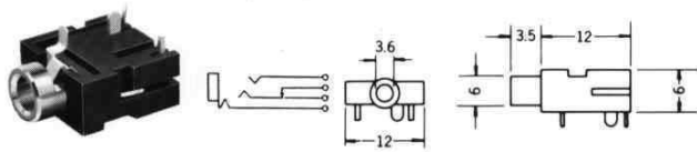
No.MJ-158L PANEL MOUNT 3-CON. STEREO MINIATURE JACK. (SINGLE CLOSED) Net Weight : 2 gr. ( \phi 3.5 )
