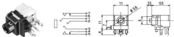
No.M03-610 ( \phi 3.5 ) STEREO
