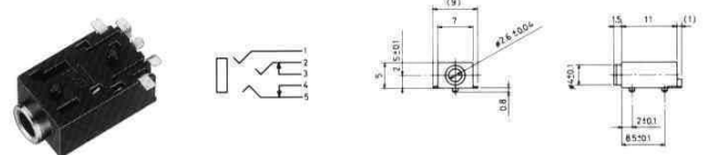
No.MJ-2-348A0 (φ2.5) With Metal Sleeve No.MJ-2-348B0 (φ2.5) Without Metal Sleeve SUB-MINIATURE STEREO JACK
