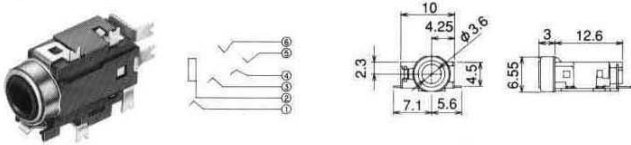
No.M03-428 (φ3.5) 6-CONDUCTOR
