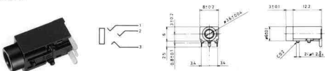
No.M03-681A0 (φ3.5) STEREO
