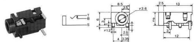
No.M03-663A0 ( \phi 3.5 ) STEREO
