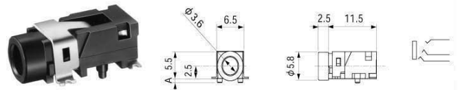
No.M03-663A0 ( \phi 3.5 ) STEREO
