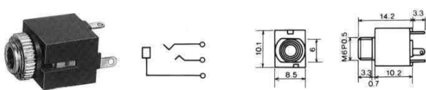
No.MJ-355W (φ3.5) CHASSIS MTG. STEREO JACK
