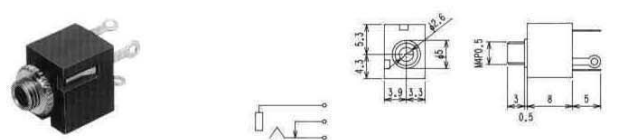
No.MJ-255 (φ2.5) MONO
