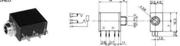
No.MJ-352W-C ( \phi 3.5 ) STEREO
