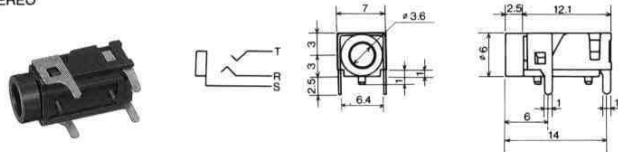
No.M03-610 ( \phi 3.5 ) STEREO
