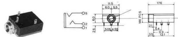
No.MJ-352W-0 ( \phi 3.5 ) STEREO
