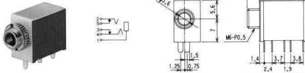
No.MJ-355 (φ3.5) MONO
