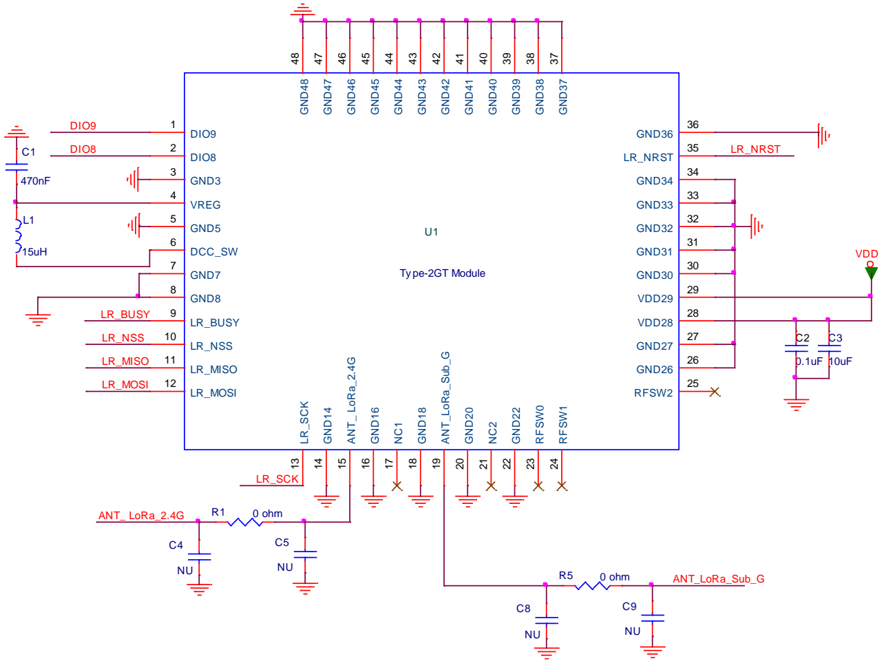
Figure 6: Reference Circuit
