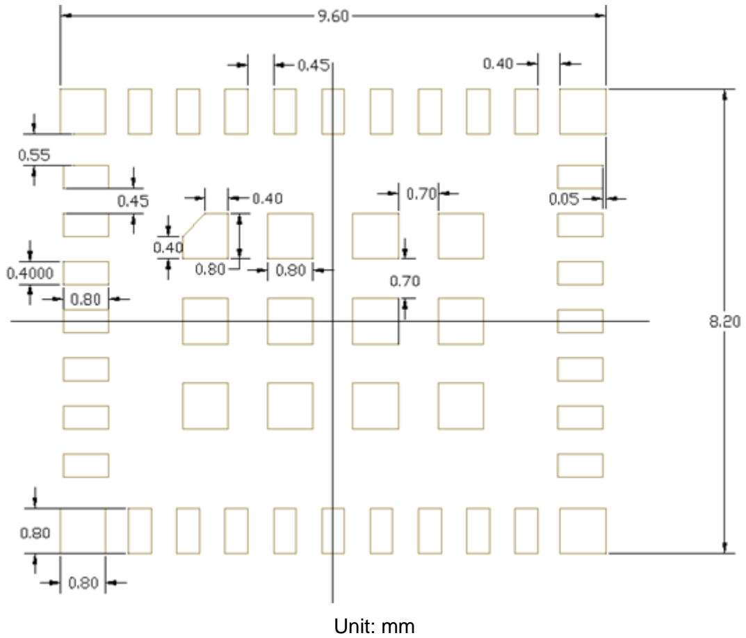
Figure 5: Land Patten
