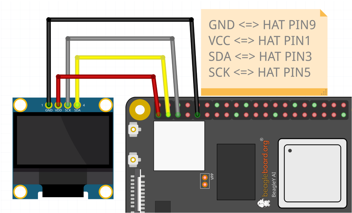
Fig. 5.17: OLED diaplay 128x64
