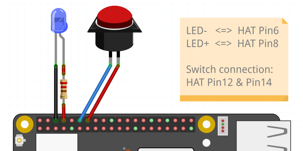
Fig. 5.7: Button connected to HAT Pin12 (GPIO18) & LED connected to HAT Pin8 (GPIO14)
