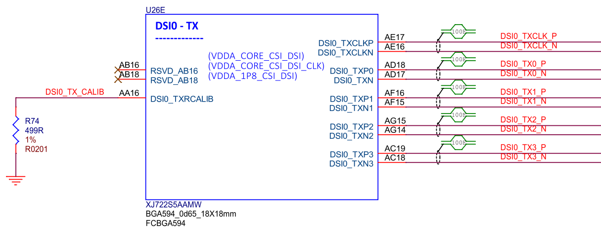
Fig. 3.53: BeagleY-AI SoC DSI0 TX connections
