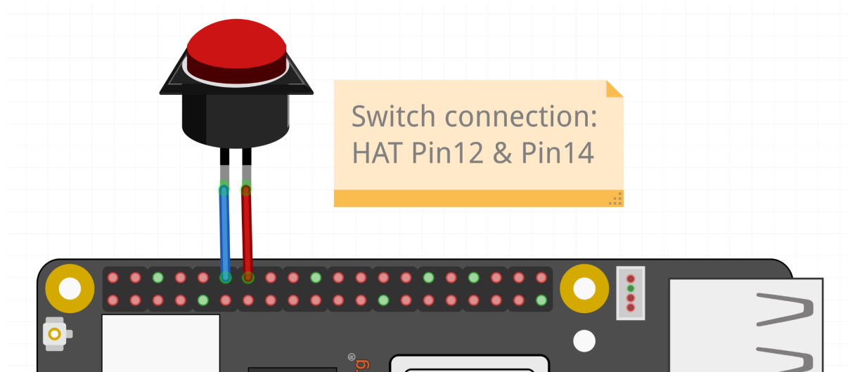
Fig. 5.6: Button connected to HAT Pin12 (GPIO18)
