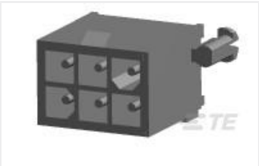
TE Part #1-770178-0 06P MINI-UMNL ASSY VO SNNI*
