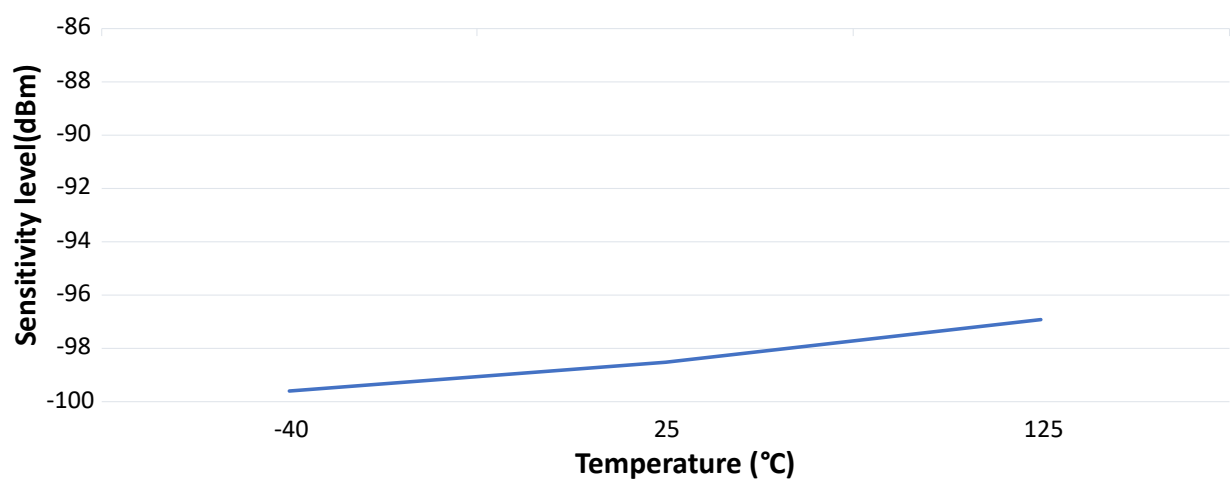
Figure 4-4. Bluetooth Low Energy Receive Sensitivity vs. Temperature
