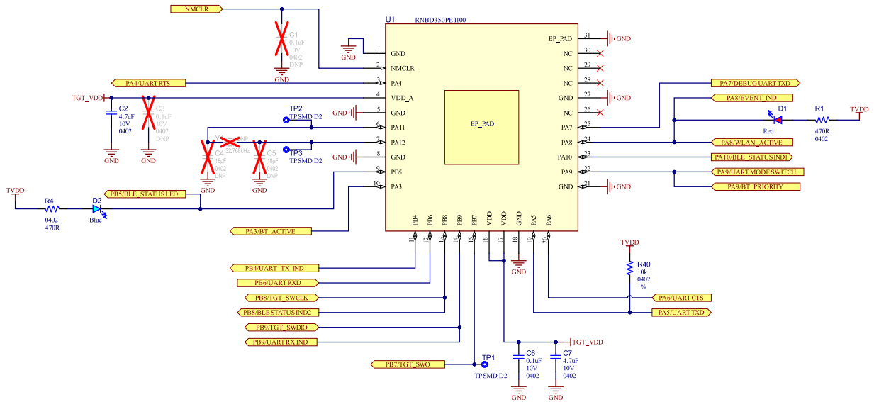
Figure 8-1. RNBD350 Add On Board
