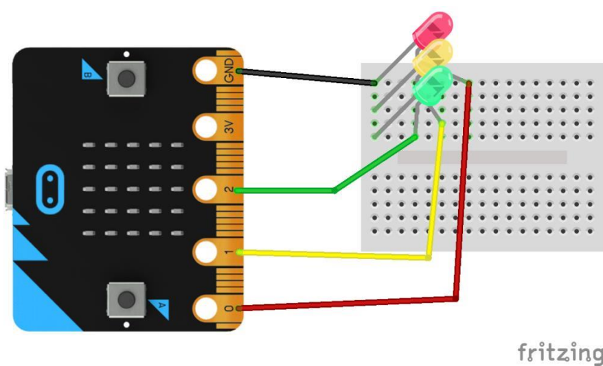
Traffic Lights Circuit
