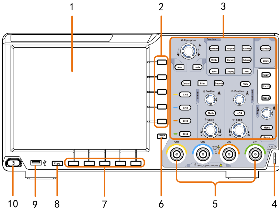
Figure 3-1 Front panel
