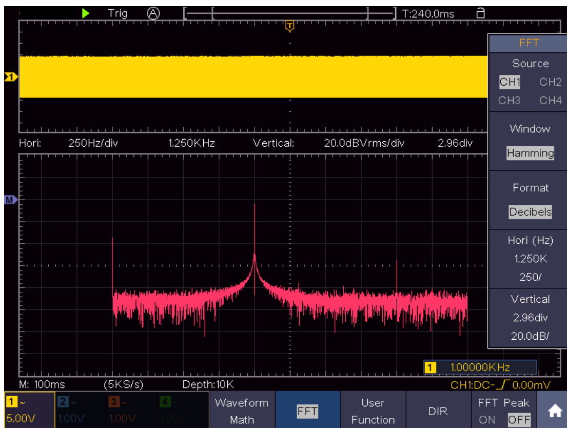
Figure 4-1 Hamming window
