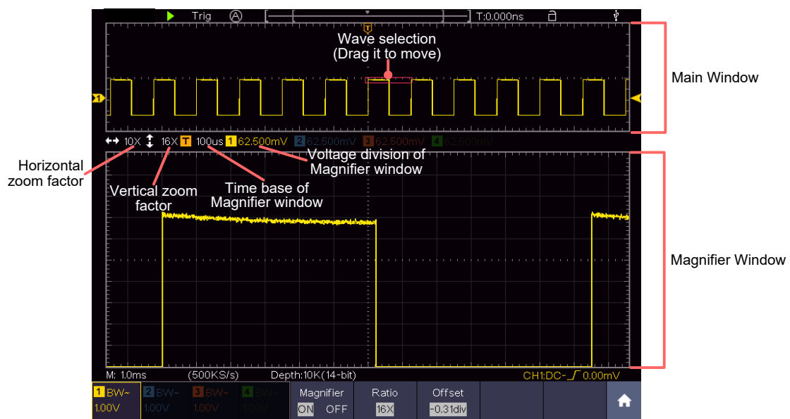
Figure 4-9 Magnifier Mode
