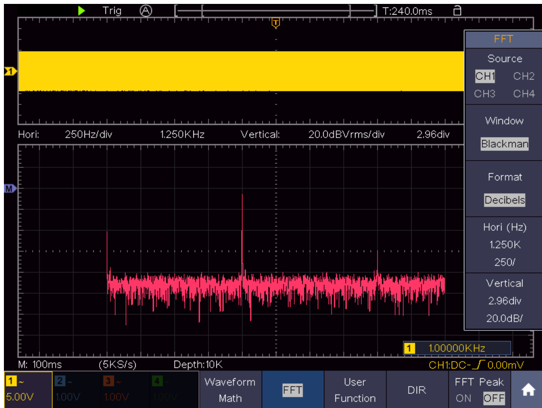
Figure 4-3 Blackman window
