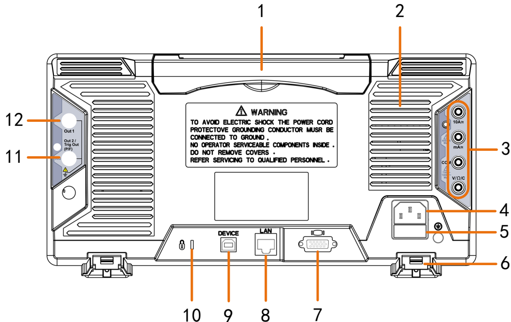
Figure 3-2 Rear Panel
