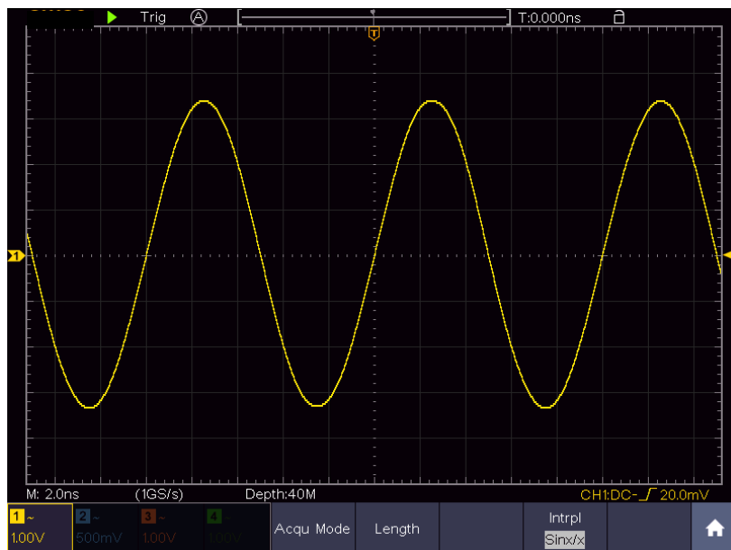
Figure 4-10 Sine(x)/x interpolation
