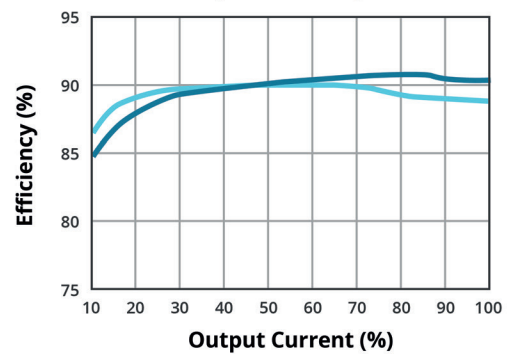
EFFICIENCY VS OUTPUT LOAD (VOF-36E-24)
