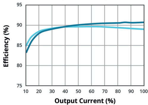
EFFICIENCY VS OUTPUT LOAD (VOF-36E-15)
