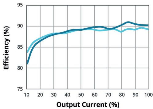
EFFICIENCY VS OUTPUT LOAD (VOF-36E-48)
