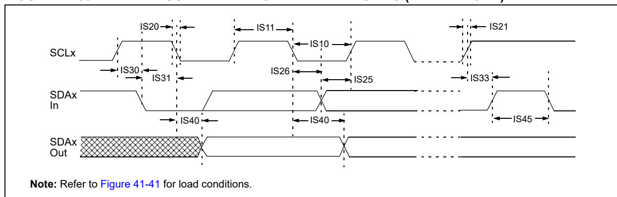
FIGURE 41-58: I2Cx BUS DATA TIMING CHARACTERISTICS (CLIENT MODE)
