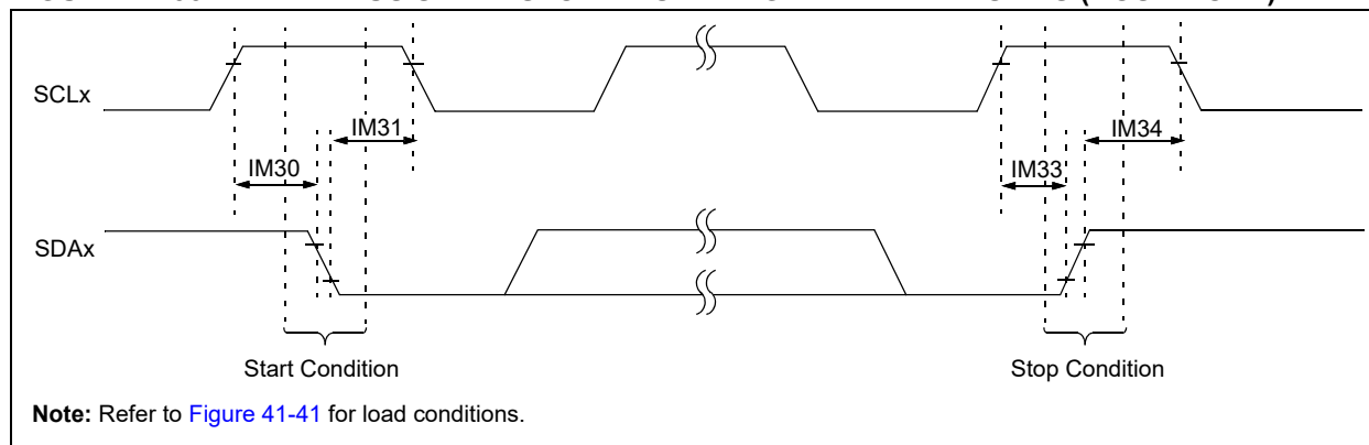
FIGURE 41-55: I2Cx BUS START/STOP BITS TIMING CHARACTERISTICS (HOST MODE)
