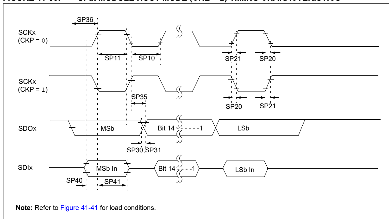
FIGURE 41-50: SPIx MODULE HOST MODE (CKE = 1) TIMING CHARACTERISTICS
