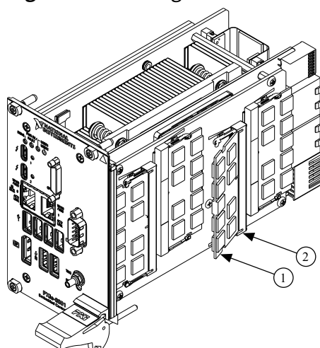
Figure 3. Installing a SO-DIMM in a PXIe-8881 Controller
