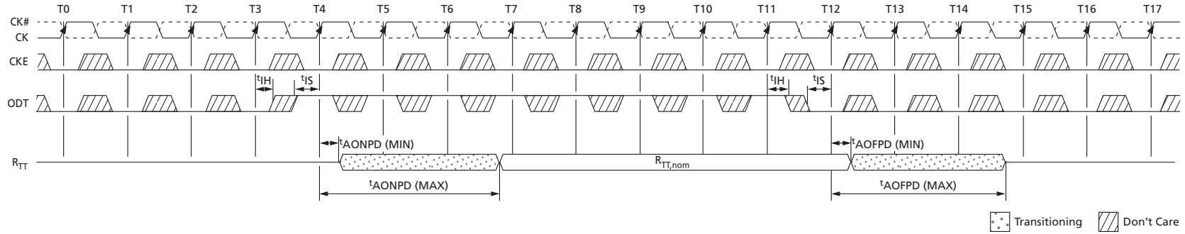
Figure 114: Asynchronous ODT Timing with Fast ODT Transition
