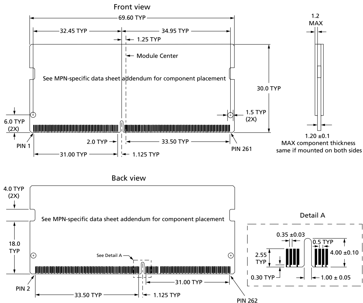
Figure 2: 262-Pin DDR5 SODIMM
