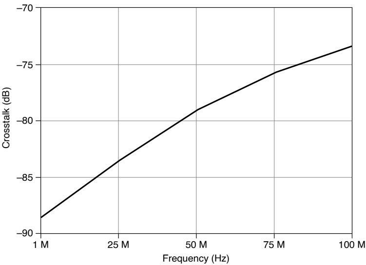
Figure 1. Channel-to-Channel Crosstalk 9
