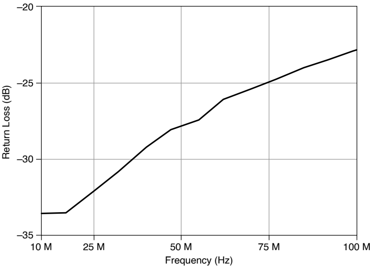
Figure 1. Input Return Loss
