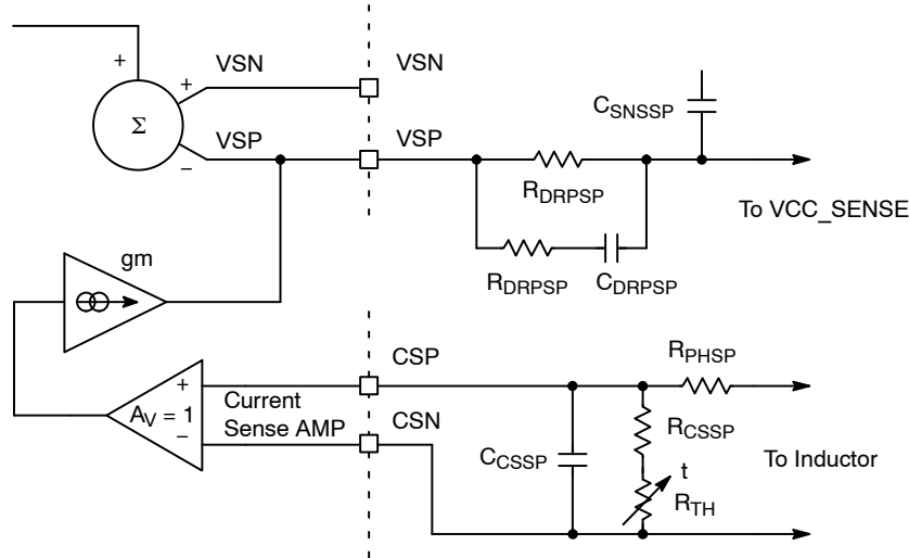
Figure 8. Load-Line Programming
