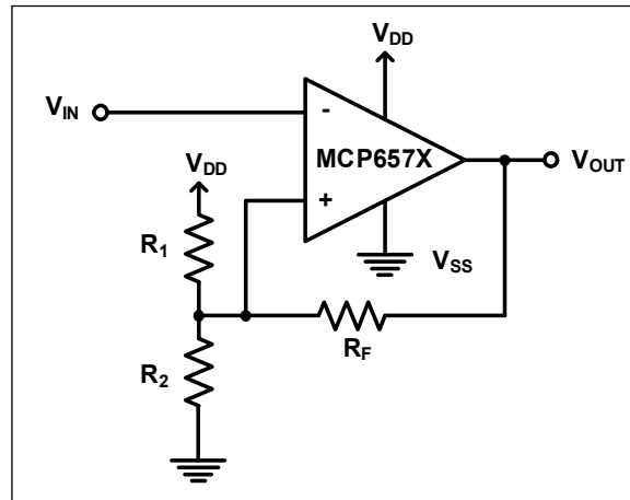
FIGURE 4-9: Inverting Circuit with Hysteresis.
