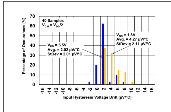
FIGURE 2-4: Input Hysteresis Voltage Drift Histogram.
