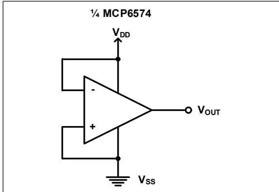
FIGURE 4-15: Unused Comparators.
