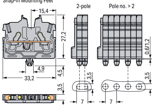
Modular Terminal Blocks and Terminal Strips with Snap-in Mounting Feet
