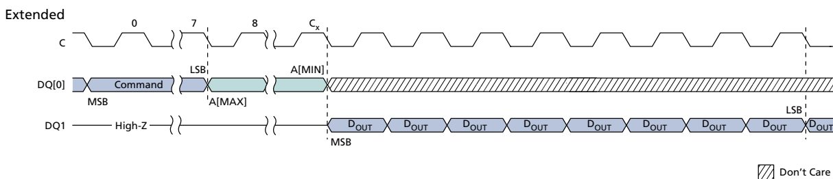
Figure 17: READ – 03h
