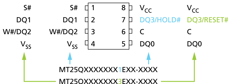
Figure 5: 8-Pin, SOP2 or W-PDFN (Top View)
