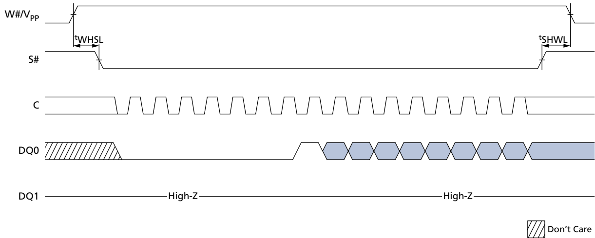
Figure 53: Hold Timing
