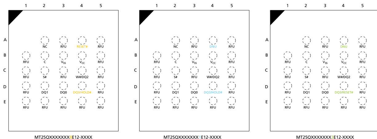
Figure 4: 24-Ball T-BGA, 5 x 5 (Balls Down)
