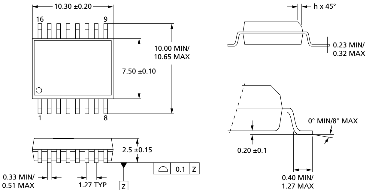
Figure 9: 16-Pin SOP2 – 300 Mils Body Width
