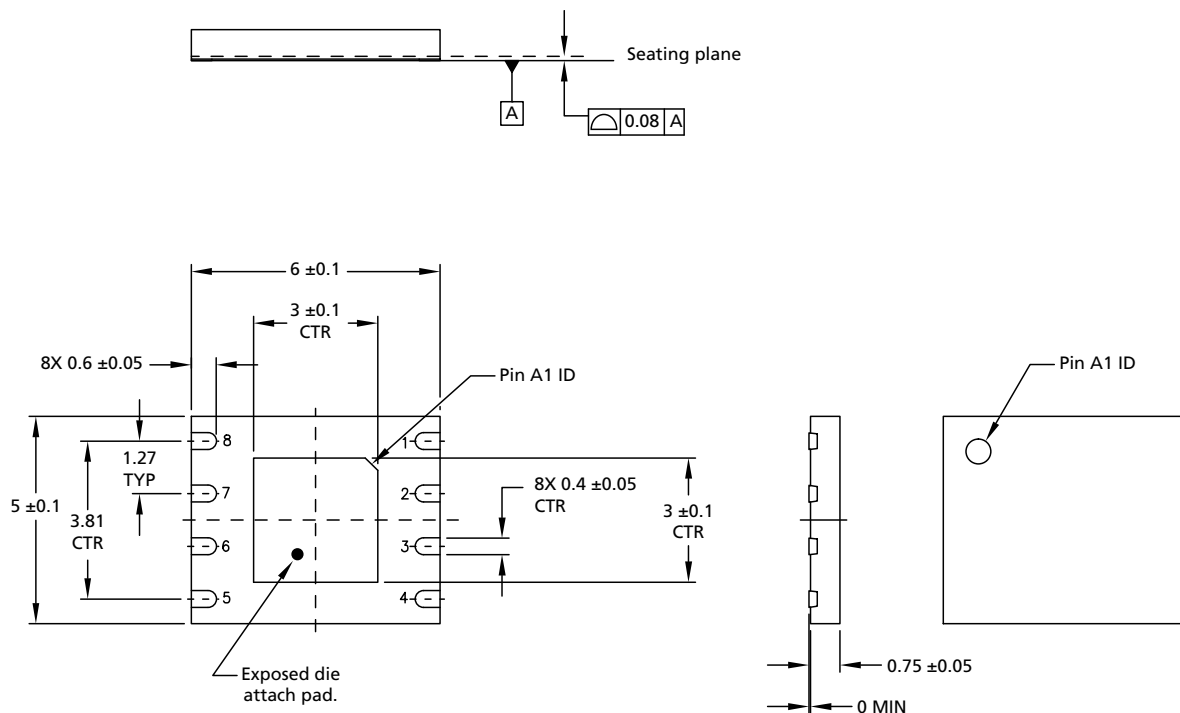
Figure 10: W-PDFN-8 (MLP8) – 6mm x 5mm
