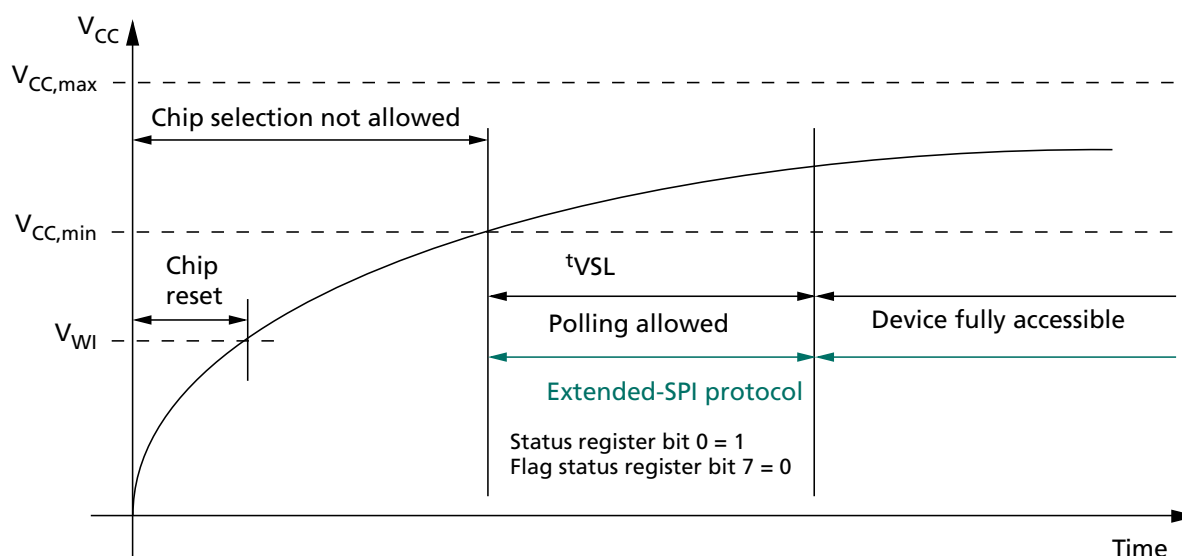
Figure 46: Power-Up Timing
