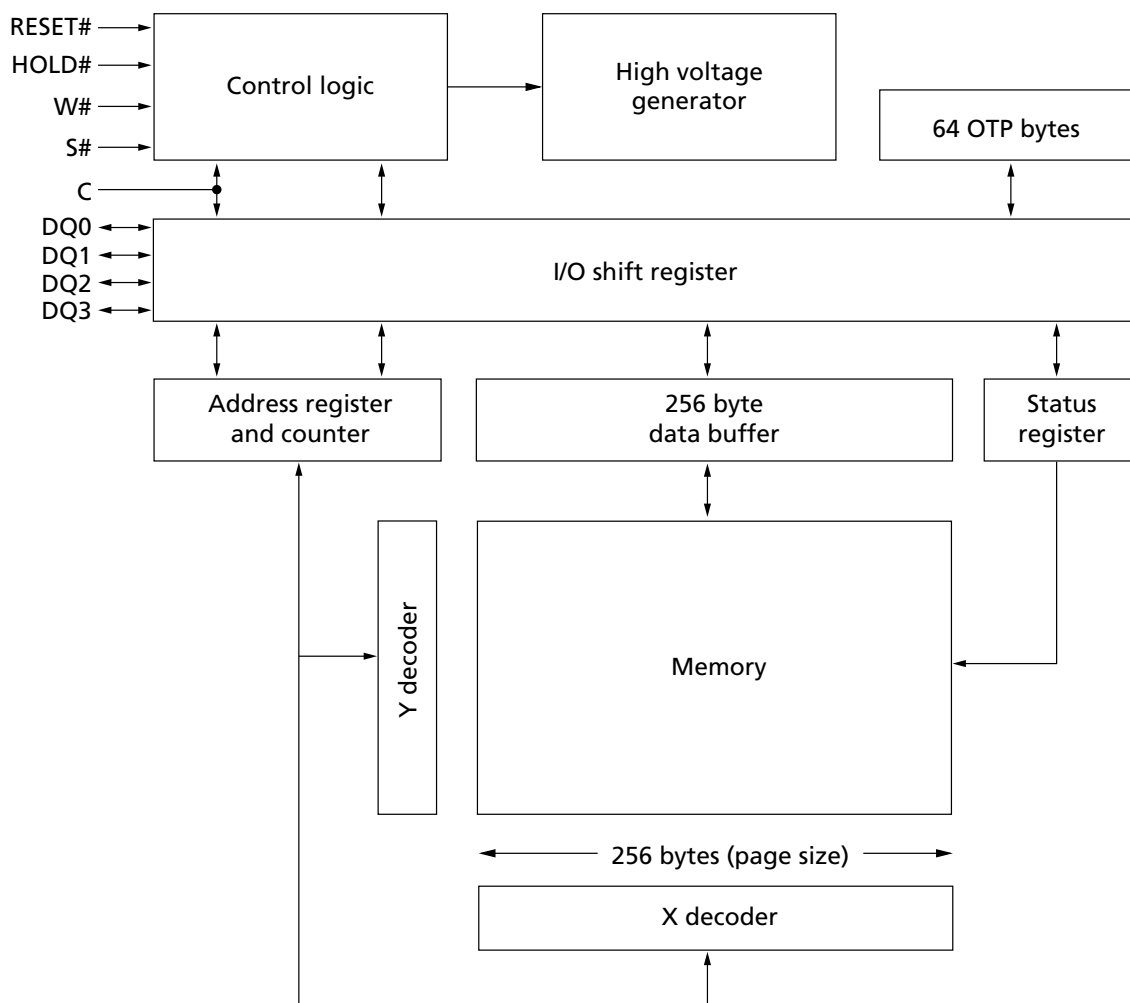
Figure 2: Block Diagram
