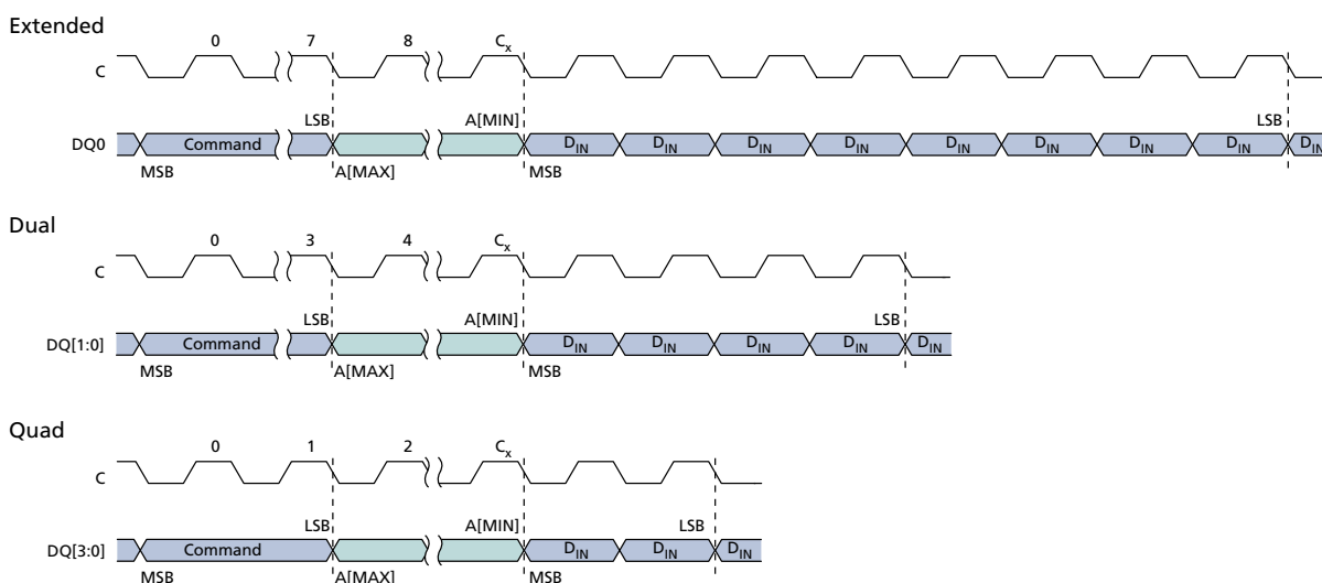
Figure 42: PROGRAM OTP Command Timing
