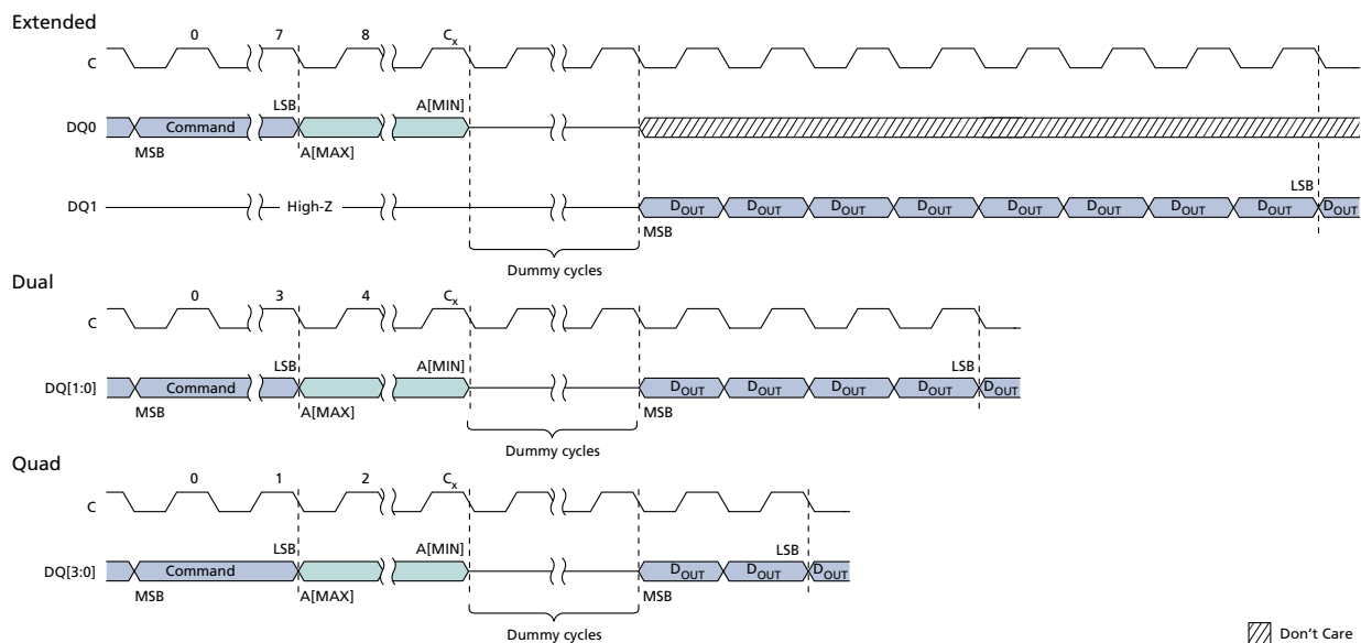
Figure 18: FAST READ – 0Bh
