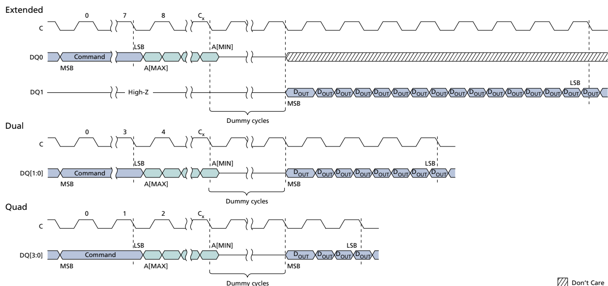
Figure 24: DTR FAST READ – 0Dh
