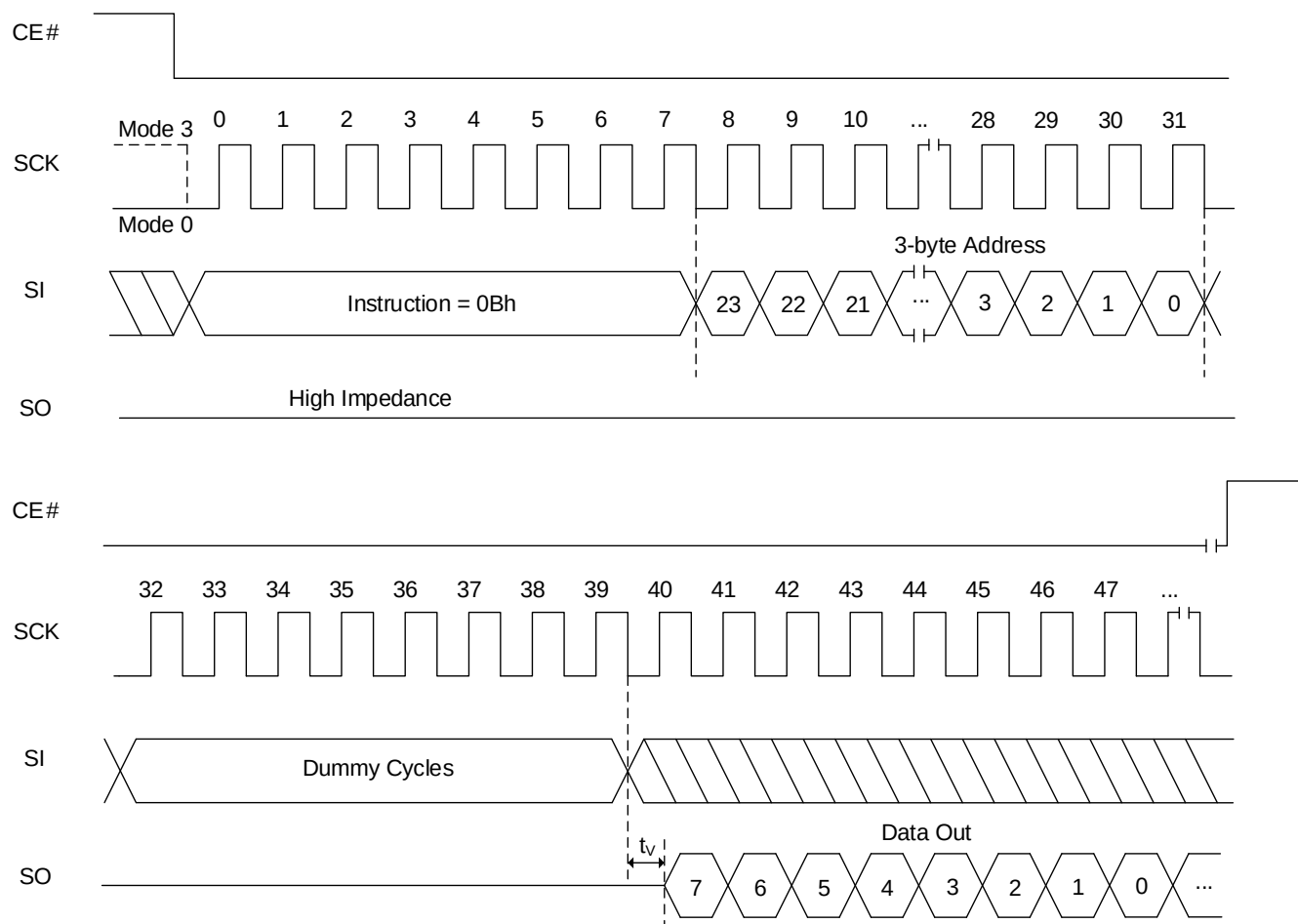
Figure 8.3 Fast Read Sequence (0Bh [EXTADD=0], 3-byte address)
