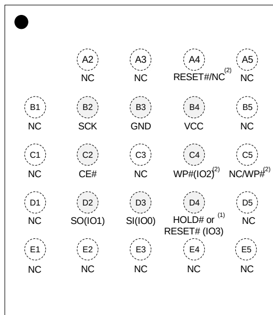
24-ball TFBGA 6x8x1.4mm (5x5 ball array) (Package: I)
