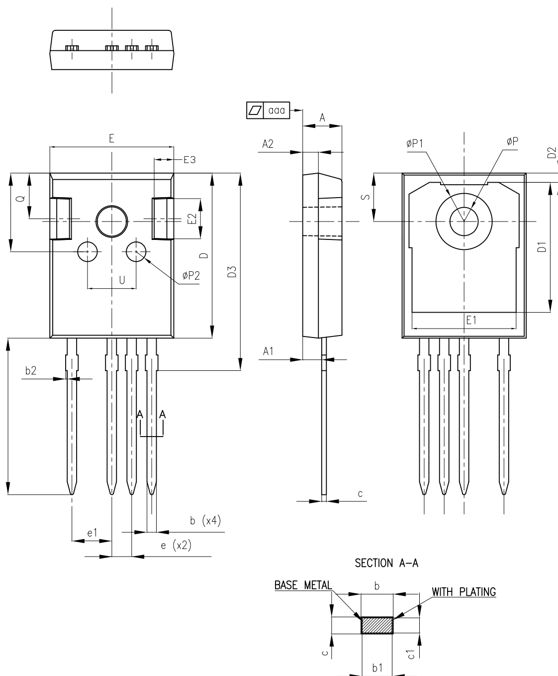
Figure 17. HiP247-4 package outline
