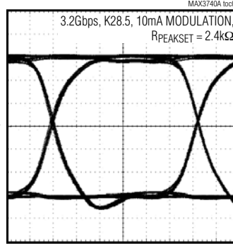
ELECTRICAL EYE WITH PEAKING
