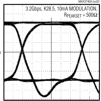
ELECTRICAL EYE WITH MAX PEAKING
