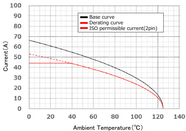
Derating Curve
