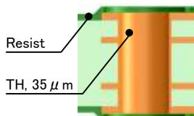
Board Layer Configuration
