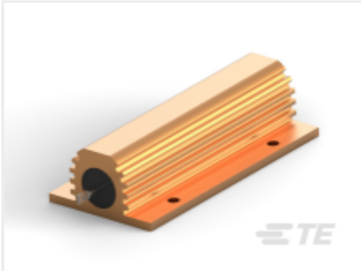
TE Part # 5-1630012-0 HSC150 22R 1%
