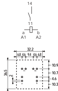
Copper side view h = 42 mm
