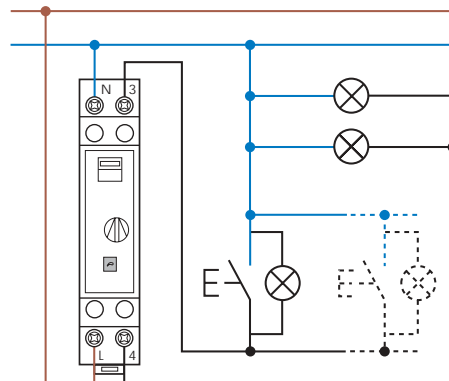
3 wire connection
