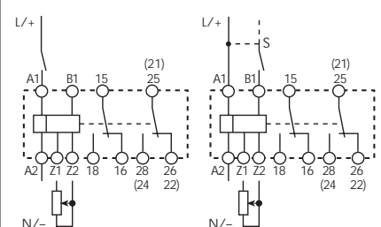
wiring diagram (without signal START)
