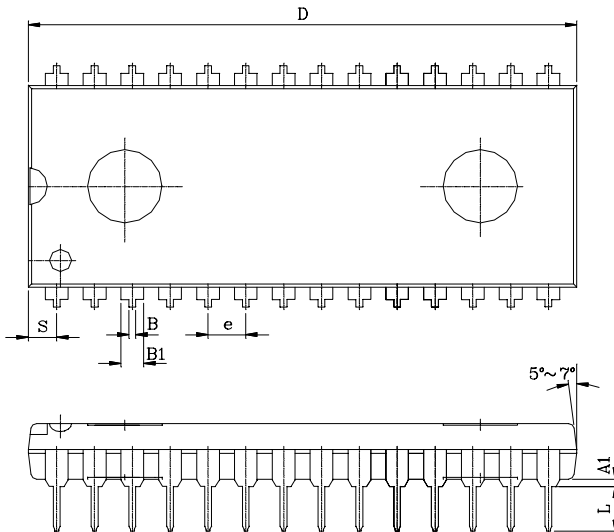
PDIP - 28
